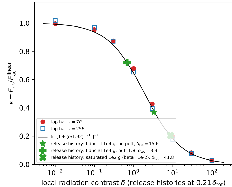
Sound efficiency of a cluster burst
