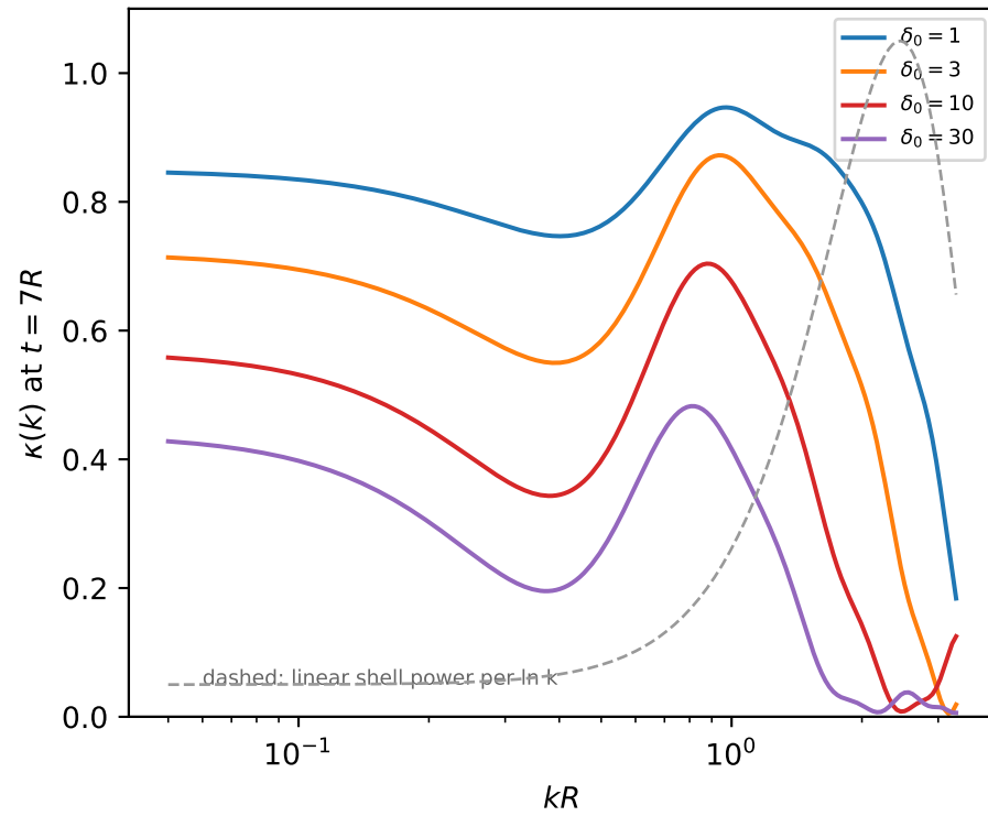
Scale dependence across the shell spectrum
