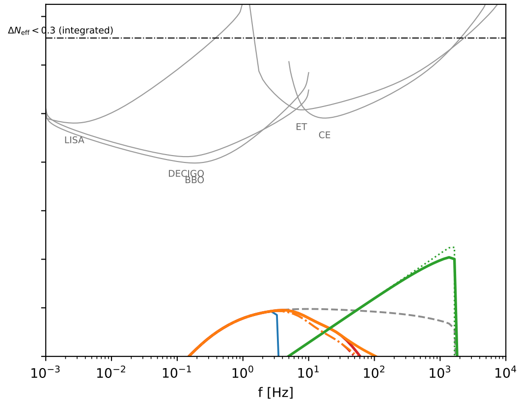
Choptuik (critical collapse): M_{\text{in}} = 10^4 \text{ g} , \beta_f = 1.1 \times 10^{-6} (published bound)
