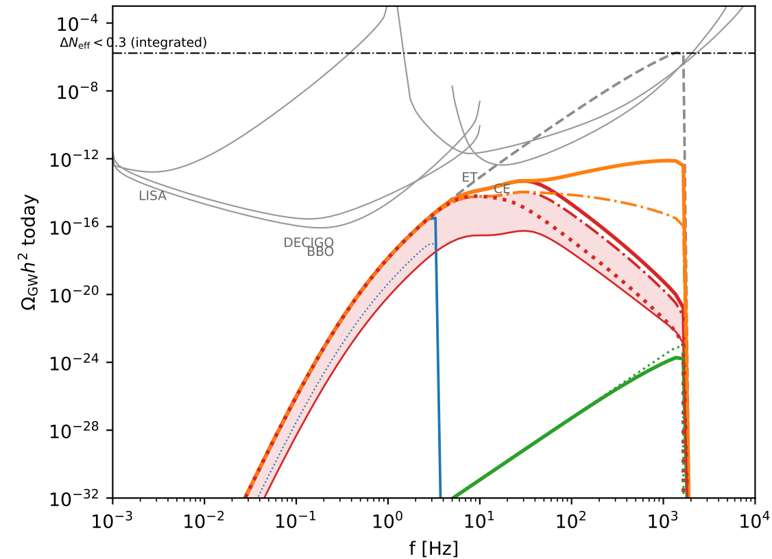
monochromatic: M_{\text{in}} = 10^4 \text{ g} , \beta_f = 1.1 \times 10^{-6} (published bound)
