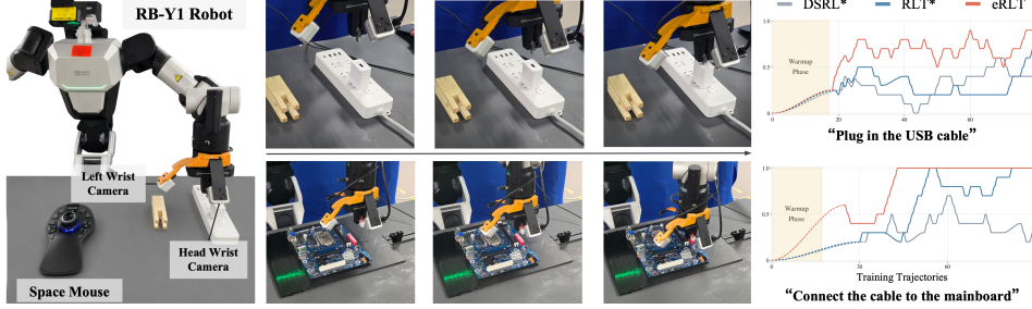
Figure 5: Real-world experimental setup and online learning curves. The RB-Y1 robot setup (left), representative execution sequences for USB connector insertion (top center) and motherboard ribbon-cable insertion (bottom center), and the 10-trajectory rolling success rate versus the number of training trajectories for both tasks (right). The shaded region marks the warm-up phase.
