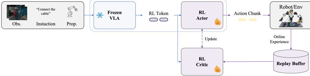
Figure 6: Lightweight online RL with a frozen VLA. A frozen VLA and a lightweight actor jointly generate executable action chunks. Online interactions train the lightweight critic and actor, and the RL token supplies task-specific action-relevant information to both modules.
