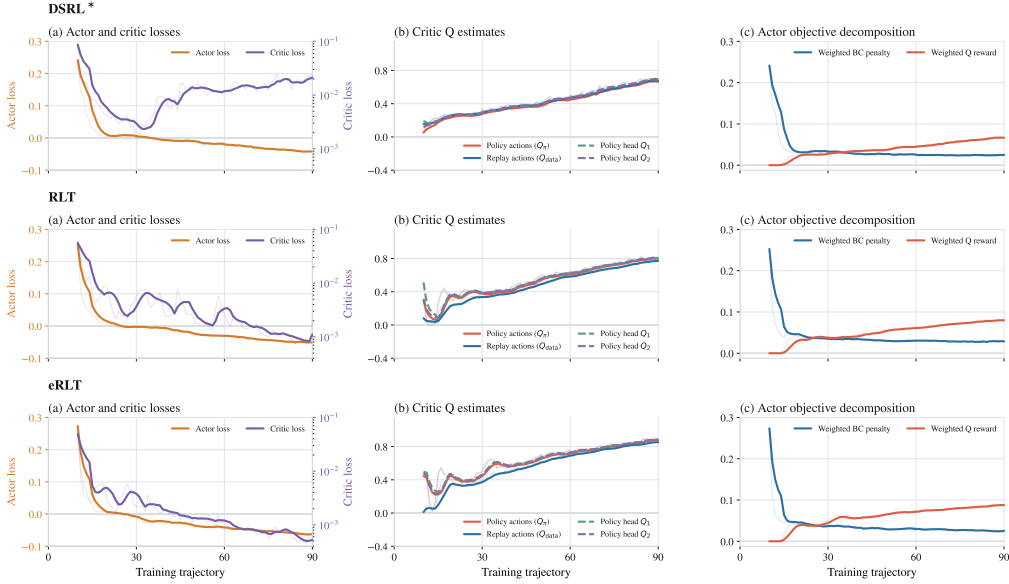
Figure 9: Online optimization dynamics for ribbon-cable insertion. Rows correspond to DSRL*, RLT, and eRLT, using the same metrics and smoothing convention as Figure 8.
