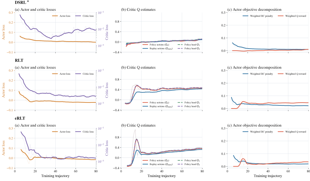
Figure 8: Online optimization dynamics for USB connector insertion. Rows correspond to DSRL*, RLT, and eRLT. Within each row, the panels show (a) actor and critic losses, (b) critic Q estimates for policy and replay actions, and (c) the weighted behavior-cloning and Q terms in the actor objective. Faint curves denote raw logged values and solid curves denote trailing-five-trajectory means.
