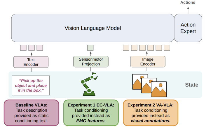
Fig. 1. An overview of vision-language-action (VLA) model architectures and how we propose to modify the inclusion of task information.
