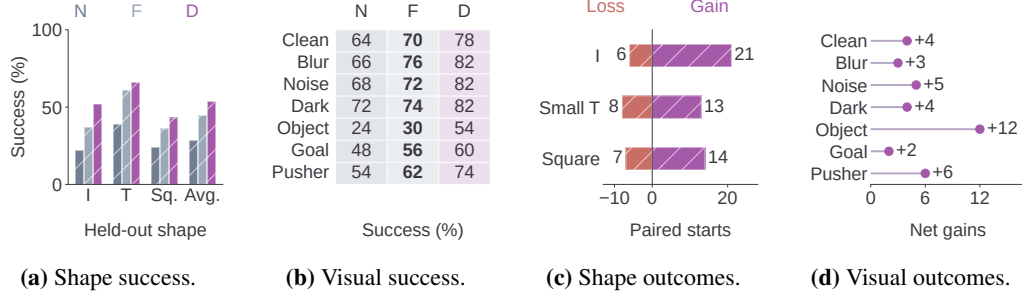
Figure 9: Decision alignment under geometric and visual change. (a) Grouped success bars and (b) a condition-by-method success matrix compare native selection (N), calibrated fusion (F) and D-JEPA (D). (c) Diverging bars separate gains from losses; (d) lollipops show their net difference relative to fusion. Each displayed group has positive net gain.
