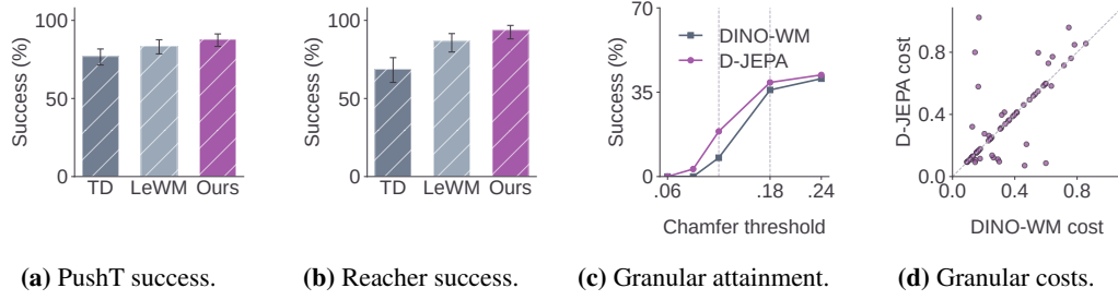
Figure 14: Executed outcomes across the formal task populations. (a,b) PushT ( n = 256 ) and Reacher ( n = 128 ) success, with Wilson 95% intervals over starts; TD denotes TD-JEPA and Ours denotes D-JEPA. Configurations match Table 1. (c) Granular success across the registered Chamfer thresholds, with strict/main thresholds at 0.12/0.18. (d) All 64 paired Granular costs; points below the diagonal favour D-JEPA. Thresholded attainment and the full cost distribution describe complementary outcomes.
