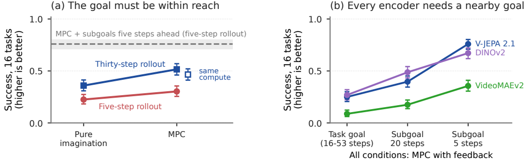
Figure 4: Keeping the target within the imagined rollout improves planning success. (a) V-JEPA 2.1 on the sixteen main tasks, planning towards a goal image from the same episode with a five-step (red) or thirty-step (blue) rollout, in pure imagination or with MPC. The open square uses the same computation as the five-step planner; the filled thirty-step points use six times more. The dashed line and grey band show MPC with a five-step rollout and subgoals five steps ahead. (b) Three encoders with MPC and a five-step rollout, planning towards a goal image from another reset or towards subgoals twenty or five steps ahead. Subgoals come from an expert rollout of the same episode.
