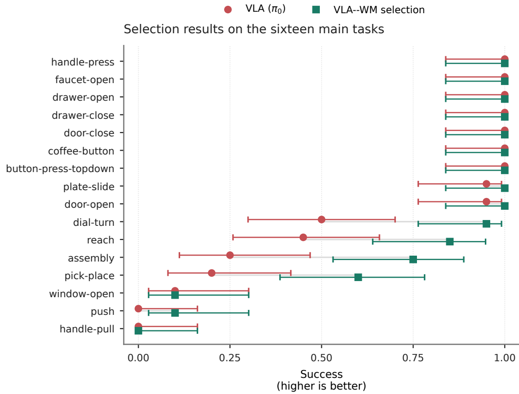
Figure 19: Per-task success of VLA and VLA--WM across the sixteen main tasks. Each task uses twenty episodes; horizontal error bars show 95% Wilson intervals.
