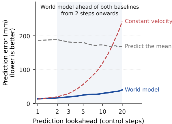
Figure 8: Decoded object-position error versus prediction lookahead for V-JEPA 2.1 and two baselines, constant velocity and predict-the-mean. Lower is better.
