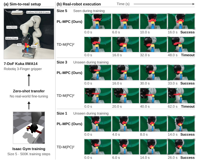
Fig. 1. Zero-shot real-robot wrench–nut alignment. (a) PL-MPC is trained entirely in Isaac Gym and deployed on a KUKA IIWA14 without real-world fine-tuning; the deployed checkpoint is selected within the first 500K training steps. (b) Representative trials on the training size (size 5) and unseen sizes 3 and 1. Frames are sampled at different times during each execution and are not consecutive control steps. In the shown size 5 and size 3 trials, PL-MPC completes the task while TD-M(PC) 2 reaches the 128-step limit. On size 1, both methods succeed, with PL-MPC completing the trial in fewer control steps. Successful sequences end with the wrench seated around the nut.
