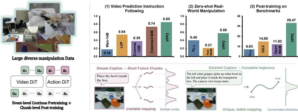
Figure 1: A typical robot policy maps an simple instruction and an observation into an short action chunk. As datasets scale, this mapping becomes increasingly multi-modes and uncertain, leading models to learn spurious short-horizon correlations. VPP2 first establishes consistent semantic-to-trajectory mappings via next event video prediction with detailed caption, then post-train and distill model to generate short action chunk.
