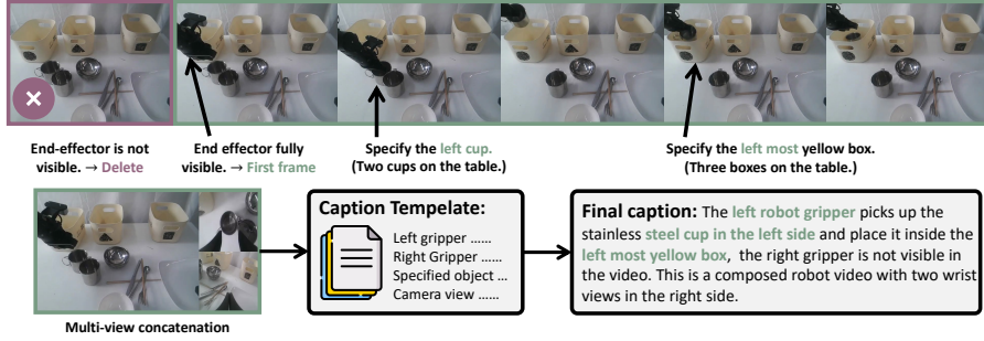
Figure 2: An example of our data process pipeline. The central objective is to reduce uncertainty in future prediction, thereby encouraging the model to learn a consistent mapping from conditioning information to sub-task trajectories. To this end, each caption includes detailed task descriptions, explicit End-Effector Identification, visible target object, and camera-view changes.
