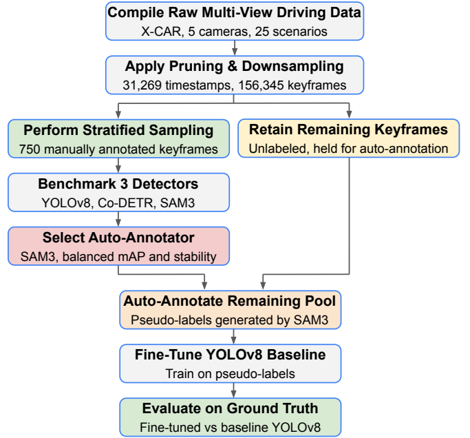
Fig. 1. End-to-end framework of the proposed foundation-guided perception pipeline.
