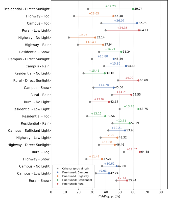
Fig. 3. Performance improvements (mAP 50-95 ) of the SAM3-guided fine-tuned YOLOv8 model versus the pre-trained baseline, sorted by the magnitude of improvement. Grey markers indicate the baseline accuracy, while colored markers denote the fine-tuned model across all 25 scenarios.
