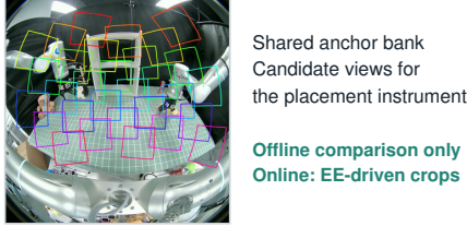
Figure 2: Observation construction and policy integration. (a) Current end-effector (EE) poses and a causal velocity estimate predict the viewing centers. Calibrated projection locates these centers in the captured fisheye image; inverse perspective sampling extracts and rectifies each local view in one step. A resized global view retains the scene. The three views enter the vision encoder, and their source rays supply a common geometric reference before action prediction. The standalone sphere illustrates the shared optical center; the grid inset uses an equidistant fisheye projection. (b) Candidate-view footprints for the offline placement instrument, selected from a shared anchor bank. These are measurement candidates, not the deployed policy inputs; online crops follow the EE poses in (a). (c) Larger views of handheld collection and the matched grippers show how tracked human poses supply the same rendering input. This interface uses pose-dependent local views while preserving global coverage.
