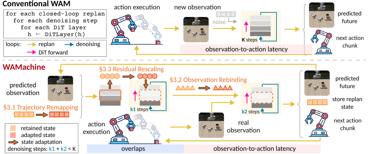
Figure 1: The main idea of WAMACHINE. WAMACHINE adapts state across replans, denoising steps, and Transformer layers to reduce computation and observation-to-action latency. K denotes native denoising steps; k_1 and k_2 denote steps before and after real observation arrival, respectively; k_1 + k_2 < K describes the illustrated accepted warm-start path.
