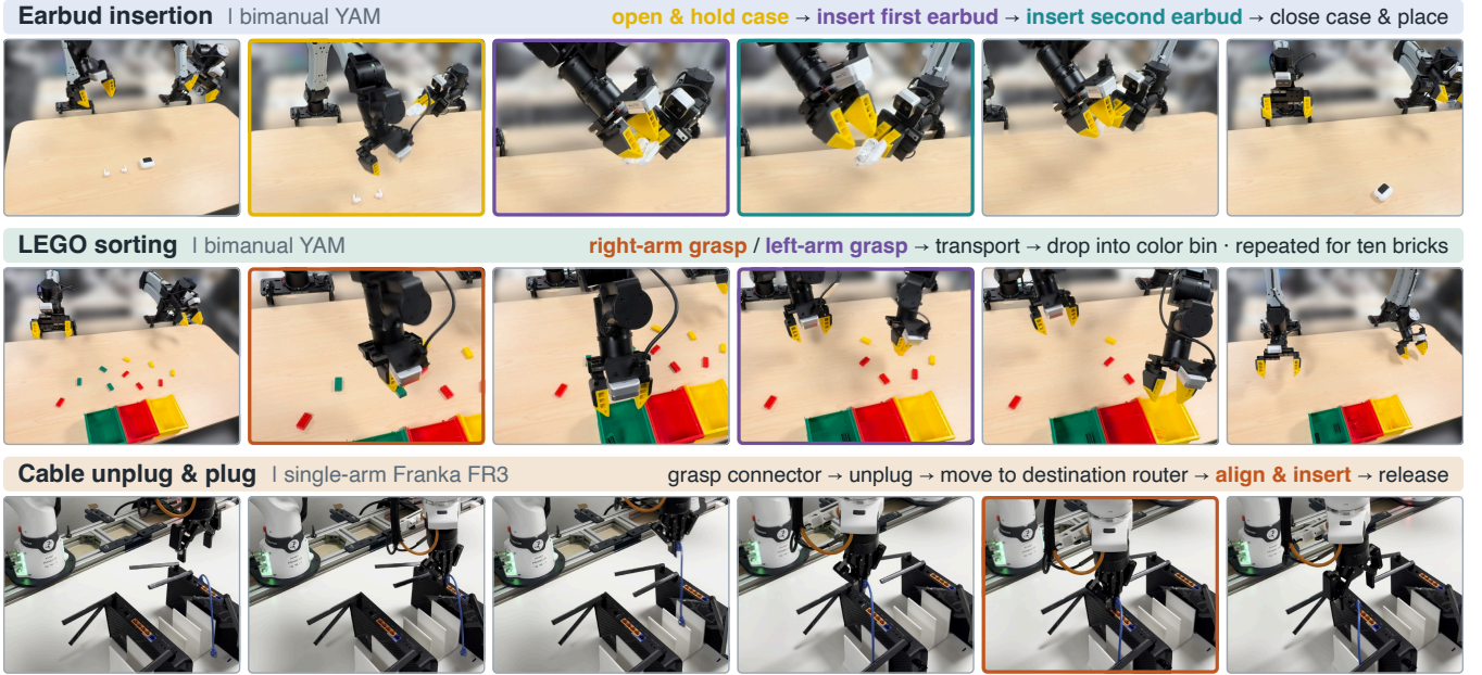
Fig. 3. Tasks on bimanual YAM and single-arm Franka FR3. Colored borders mark states produced by a targeted residual policy, in the color of its subtask name in the row header. Top : earbud insertion, where inserting earbuds requires high precision. Middle : LEGO sorting, where the grasp of each small brick is the recurring bottleneck because the brick size is out-of-distribution for the base policy. Bottom : cable insertion requires precise manipulation.
