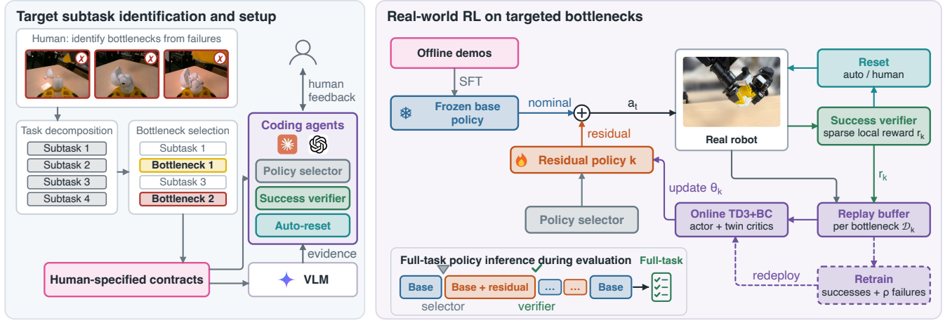
Fig. 2. PARTS architecture. Left : Humans identify bottlenecks from base-policy failures and specify contracts. Coding agents implement selection, verification, and reset programs. Right : Residual policies correct the frozen base policy. Local rewards and per-bottleneck replay support online TD3+BC and retraining on all successes plus a fraction \rho of failures. Retrained policies resume online learning. At evaluation, PARTS enables the switch between the base and residual policies to complete the full task.
