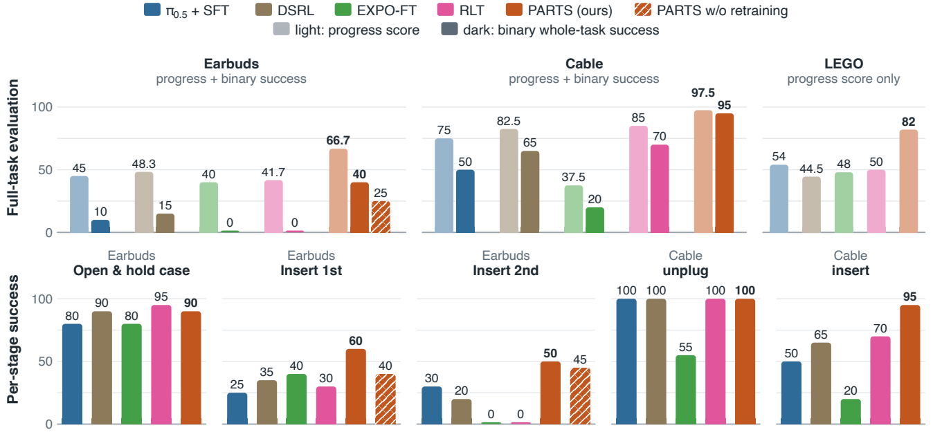
Fig. 4. PARTS significantly raises success across tasks with different difficulty levels and outperforms RL fine-tuning baselines under a matched robot-robot budget. Top : full-task evaluation over 20 episodes per method; for each method the light bar is the progress score and the dark bar is binary whole-task success. Earbud progress credits one third per completed stage and success requires all three; cable progress credits one half each for unplugging and insertion and success requires both. LEGO is a repeated pick-and-place task over ten bricks, so we report only its progress score, the fraction of bricks sorted before the deadline, which is more informative than a binary outcome over the whole task. The ablation is reported for binary success only. Bottom : per-stage success measured within the same episodes, for the three earbud bottlenecks and the two cable stages. Hatched bars are PARTS without success-reweighted retraining.
