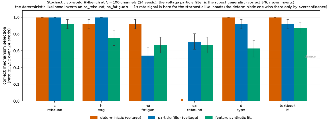
Figure 28: Three observation models on the stochastic six-world battery (fixed hypothesis space) ( N=100 channels; correct-selection rate \pm 1 SE over 24 seeds; a dot marks an exact zero). The voltage particle filter (blue) is the robust generalist — correct on five of six worlds and never inverting (its one weak world is the SNR-limited NA-FATIGUE, at chance). The deterministic likelihood (orange) inverts on CA-REBOUND (wrong on every one of the 24 seeds). The feature synthetic likelihood (green) stays above chance on every world and edges the particle filter on the rate world NA-FATIGUE, but is weaker on the worlds whose discriminating signal is a sub-threshold or timing shape (H-SAG, D-TYPE) that the summary vector compresses. On NA-FATIGUE only the deterministic likelihood is clearly correct; however the deterministic likelihood catastrophically fails (inverts) on CA-REBOUND.
