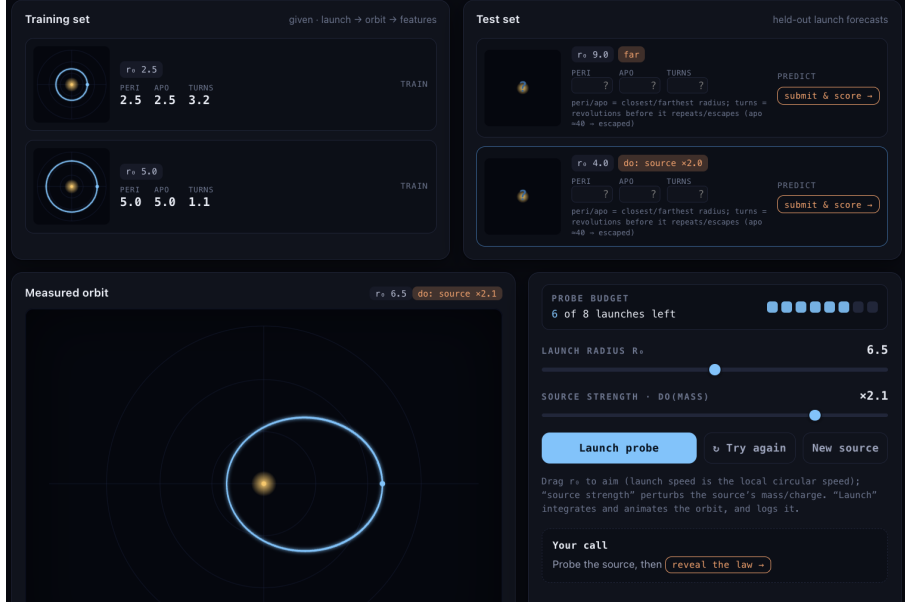
Figure 6: App for FORCEBENCH. The goal is to identify a hidden central-force law from a few probe orbits, then predict held-out launches — including one under a perturbed source. Training orbits (top left), held-out interventional test forecasts (top right), and the reader’s own budgeted experiment bench with an animated measured orbit (bottom). Available at https://claude.ai/code/artifact/565fe6cc-a355-4c19-bf7e-b44e766cf87e .
