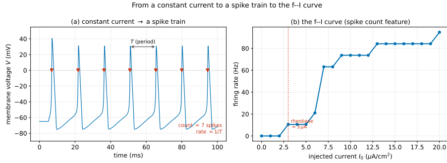
Figure 17: The f-I curve, and why we count spikes. (a) A constant supra-threshold current makes the model fire a periodic spike train ; the readout is simply the spike count (red markers) — or, per unit time, the firing rate 1/T . (b) Sweeping the injected current traces the f-I curve (firing rate vs. current): flat and zero below the rheobase (the smallest current that fires, red), then rising. This matches the intuitive “how many spikes” readout.
