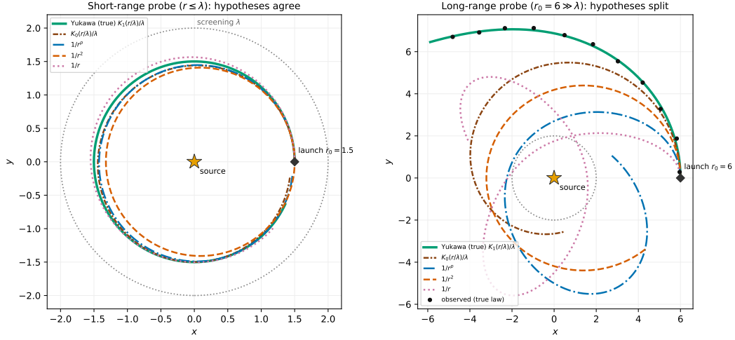
Figure 14: Probe orbits under the candidate force laws for YUKAWA world: a short-range vs. a long-range design. The screened Yukawa kernel K_1(r/\lambda)/\lambda and the power laws fit to the short-range seed data nearly coincide for r \leq \lambda and diverge only beyond it. ( left ) Launched within the screening length ( r_0=1.5 ), every candidate law traces almost the same orbit — they cannot be told apart. ( right ) Launched well beyond it ( r_0=6 , matching the long-range probes of Fig. 1b): the true screened kernel (green, with the observed data) has decayed, so it holds a wide slow arc, whereas the un-decayed power-law near-misses are far too strong at this range and plunge inward — the hypotheses fan out.
