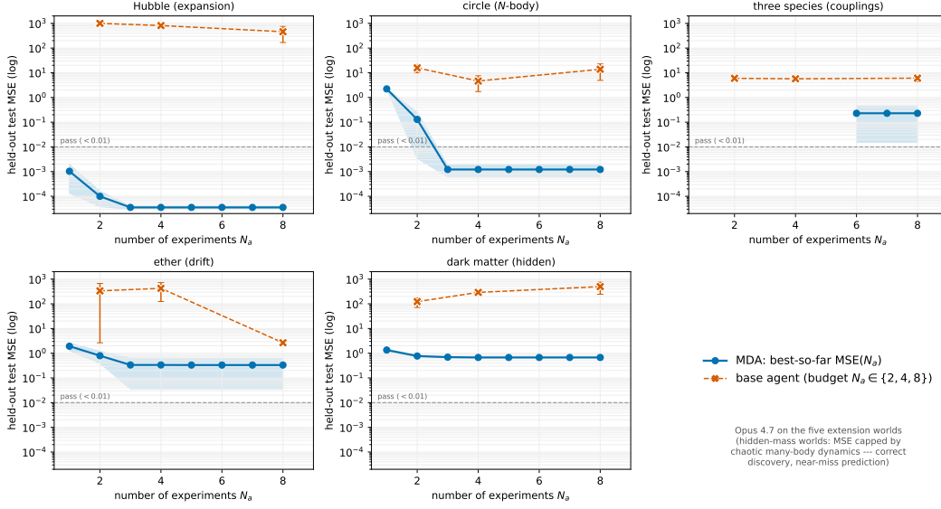
Figure 8: Data efficiency on MULTIPARTICLEWORLDS using Opus 4.7. We plot held-out forecast MSE vs. experiments for MDA (solid, mean \pm SE over seeds) against the pure agent (dashed). MDA is orders of magnitude better at every budget. Several worlds clear the pass line (error of 0.01 or less) within three experiments. Ether and dark matter plateau above the line, but this is the intrinsic ceiling of their scoring (due to near-singular free-fall and a chaotic many-body system), not a discovery failure (since MDA recovers the correct drift and the hidden monopole).
