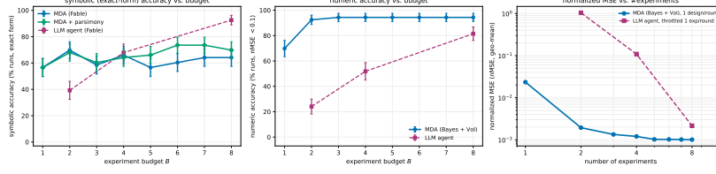
Figure 12: Data-efficiency curves with the strongest base model (Table 5) on both arms , aggregated over all six FORCEBENCH worlds. (left) Exact-form accuracy vs. budget: the parsimony submission (green) lifts MDA (blue) toward the strong unaided agent (purple), which leads on pure structure recovery. (middle) Numeric accuracy (fraction of runs with normalized MSE < 0.1): MDA reaches \sim 94\% within \sim 3 designed experiments and dominates the agent everywhere. (right) Normalized MSE vs. number of experiments: MDA converges to \sim 10^{-3} in \sim 2 experiments, an accuracy the throttled agent reaches only by B=8 . So even against a strong proposer, MDA's Bayesian inference on the same proposals never hurts and sharply helps on the predictive metric. Error bars are \pm 1 SE over the 9 runs ( 3 seeds \times 3 LLM draws) per world.
