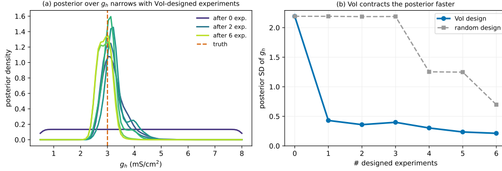
Figure 24: Parameter refinement on NEURONBENCH (H-SAG world: a hidden hyperpolarisation-activated I_h current, the second half of the discover-then-refine loop begun in Fig. 23). Once the mechanism is identified, its maximal conductance g_h is inferred from the Gaussian synthetic likelihood on trace features s(\theta) (the gating kinetics are held fixed, per Table 14); because the model is deterministic this likelihood needs no simulation-based estimation. (a) The posterior over g_h contracts from the uniform prior onto the truth (dashed) as Vol-designed experiments accumulate. (b) Vol — which selects the hyperpolarising probes that make the sag, and hence s(\theta) , depend on g_h — contracts the posterior standard deviation \sim 8\times in a single experiment, whereas random design, spending most probes on uninformative depolarising steps, lags several-fold. The menu here is augmented with a battery of hyperpolarising steps at different depths.
