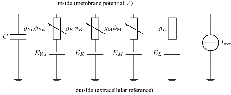
Figure 19: The Hodgkin-Huxley equivalent circuit (Eq. (21)). The membrane is a capacitor C ; each ion channel is a branch with a variable conductance g_c \phi_c (opening/closing gates \phi_c ) in series with a battery E_c (the reversal potential). The injected current I_{\text{ext}} charges the capacitor and flows through the open channels; a blocker deletes a branch ( g_c \rightarrow 0 ). Which branches are present is the structure ; the conductances g_c are the parameters .
