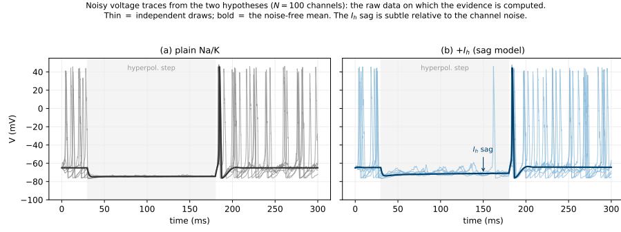
Figure 26: Stochastic-latent NEURONBENCH: the raw data. Noisy voltage traces from the two competing hypotheses under a moderate hyperpolarising-step protocol, at N=100 channels (thin: independent draws; bold: the noise-free mean). (a) A plain Na/K cell. (b) The same cell plus a hyperpolarisation-activated I_h current (the H-SAG model of Table 12), whose only signature is a small depolarising sag during the step (arrow). Because that sag is comparable in size to the channel noise, the two hypotheses overlap and cannot be told apart by eye — this is the data on which the evidence of Fig. 27 is computed.
