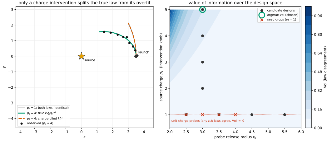
Figure 13: Visualising COULOMB world and its design space.
