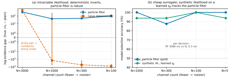
Figure 27: Stochastic-latent NEURONBENCH: estimating the intractable likelihood by simulation. Both panels score the I_h -vs-plain decision on the data of Fig. 26, sweeping the channel count N (fewer = noisier). (a) The log-evidence gap \log Z_1 - \log Z_2 vs. N . A likelihood that ignores the process noise (a single deterministic rollout + Gaussian observation, orange) degrades and, below N \approx 1000 , inverts — a negative gap means it confidently selects the wrong mechanism. A bootstrap particle filter (blue), which estimates p(y | m, \theta) by propagating the latent gating SDE, stays robustly positive. (b) A synthetic likelihood on a learned summary s_\phi (green) reproduces the particle filter’s model-selection accuracy across the noise sweep at \sim 10^4 \times less compute ( \sim 0.3 ms vs. \sim 3 s per decision). Bars/points are \pm 1 SE over independent noise realisations; see Section A.4 for s_\phi .
