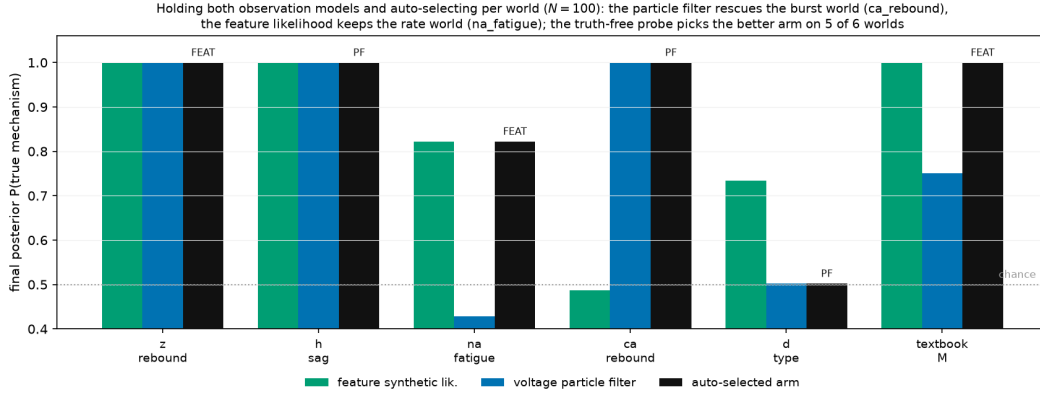
Figure 29: An auto-selected observation model ( N=100 , six worlds, fixed hypothesis space; final posterior of the true mechanism under repeat-aware VoI). The feature synthetic likelihood (green) and voltage particle filter (blue) are complementary — the PF rescues CA-REBOUND’s burst while the feature likelihood keeps NA-FATIGUE’s spike-rate signature (where the PF is below chance). The agent auto-selects (black) by a truth-free discrimination probe — which likelihood best separates the candidates on the discriminator, averaged over each candidate generating the data (the letter marks the chosen model, PF or FEAT). It attains the better arm on five of six worlds; on D-TYPE the single-shot probe favours the PF, which then underperforms the feature likelihood under the budgeted design.
