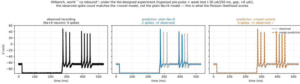
Figure 22: Visualizing the predictions of two different models on CA-REBOUND. We show the observed recording (left) and the spike response predicted by each candidate structure (plain Na+K neuron in middle, augmented model with novel channel on right) under the VoI-designed experiment. The plain Na+K neuron fires 2 spikes and misses the rebound (middle, \neq observed); the neuron with the extra current fires the 4-spike rebound burst that matches the data (right, = observed). The Poisson likelihood scores exactly this: the spike count each deterministic model predicts is the Poisson rate (Eq. (32)), so the observed count identifies the mechanism.
