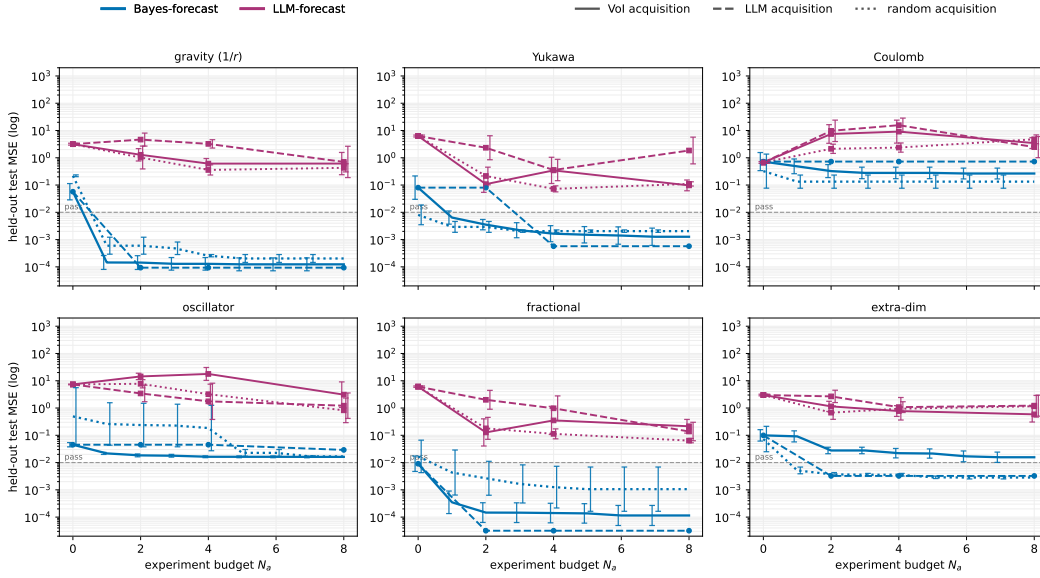
Figure 7: Per-world data efficiency on TWOPARTICLEWORLDS (Opus 4.7; the compact aggregate is Fig. 2 in the main text). One panel per world. Colour = forecaster (blue Bayes-forecast, purple LLM-forecast); line style = acquisition (VoI solid, LLM dashed, random dotted). The initial value at N_a = 0 is the result based on D_0 before any experiments. Uncertainty is \pm 1 SE in \log_{10} over 9 runs (3 random initial conditions \times 3 draws per IC): a shaded band on the continuous best-so-far Bayes-forecast/VoI traces, and error bars on the N_a \in \{0, 2, 4, 8\} budget points of both forecasters. Within the Bayes-forecaster family the VoI and LLM design strategies perform similarly and both generally beat random.
