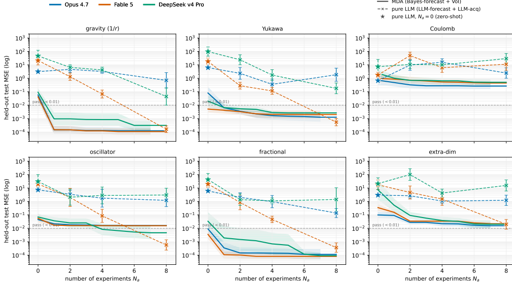
Figure 11: Effect of changing the proposer LLM on data efficiency: held-out test MSE vs. experiment budget B , per world, for three proposer LLMs (Opus 4.7, Fable 5, DeepSeek v4 Pro; colour). Solid: MDA (Bayes-forecast + Vol acquisition), the best-so-far MSE( B ) trajectory with a \pm 1 SE band. Dashed: the matched pure-LLM agent (LLM-forecast + LLM-acq) at B \in \{0, 2, 4, 8\} , with \pm 1 SE error bars and anchored at its B=0 zero-shot law ( \star ). Uncertainty is over 9 runs (3 seeds \times 3 draws), geometric mean \pm 1 SE in \log_{10} . Grey: the pass threshold (0.01). Across proposers, MDA drives the held-out error to the identifiability floor within a few experiments, whereas LLM agent behavior plateaus well above it on most worlds, except in the case of Fable.
