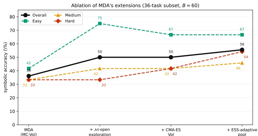
Figure 16: Ablation of MDA’s extensions beyond ModelSMC: symbolic accuracy per tier and overall, added incrementally on the 36-task subset at B=60 . Each extension helps a distinct tier. \mathcal{M} -open exploration lifts the easy tier (42→75%, single-mechanism correction; also the only route to any compound recovery) but leaves the hard tier flat; CMA-ES VoI and then the ESS-adaptive pool lift the hard tier (33→42→54% — sharper designs, then evicting the over-elaborated near-duplicates exploration introduces). The full config is the two-seed result of Table 9; intermediate configs are seed 0.
