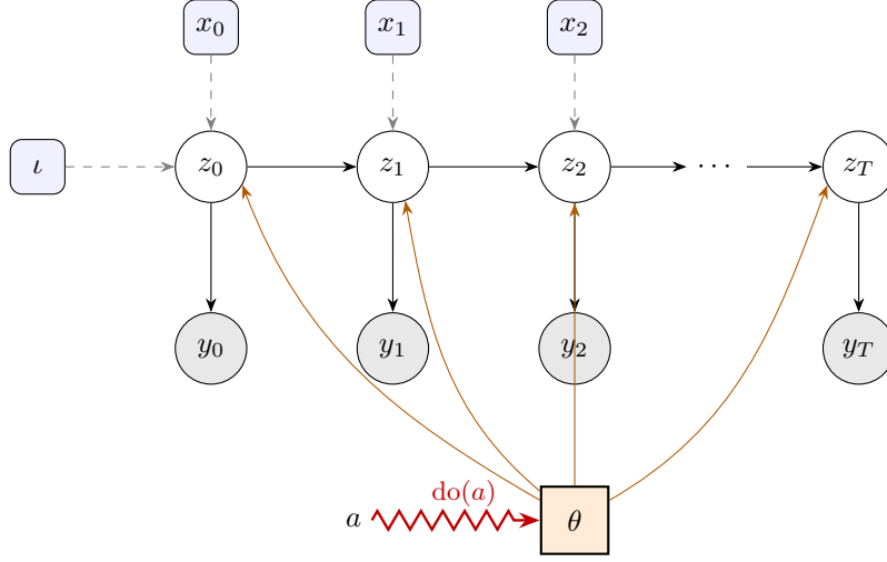
Figure 5: The world as a controlled, intervenable state-space model (Eq. (1)). A latent state z_t (white) evolves under the mechanism \theta (orange; it parameterizes every transition) and emits a lossy, noisy observation y_t (grey) — in general only y_{1:T} is seen. Optional exogenous inputs/covariates x_t (blue, dashed) and the initial condition \iota (which sets z_0 ) are shifts in the inputs to a fixed mechanism. An intervention \text{do}(a) is categorically different: the lightning bolt strikes \theta itself, changing the mechanism to \theta_a .
