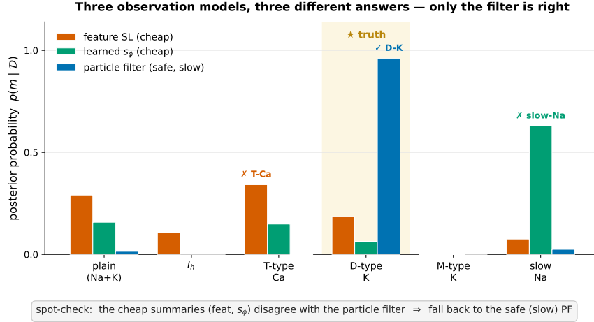
Figure 30: The particle-filter spot-check (D-TYPE, fixed archetype pool, N=100 ). The two cheap observation models disagree with each other and with the particle filter: the fixed-feature synthetic likelihood picks T-type Ca and the learned s_\phi picks slow- \text{Na}^+ , while only the assumption-free particle filter recovers the true D-type K current ( \star ). Because a selected cheap model’s MAP disagrees with a PF spot-check on the collected data, the auto-select of Eq. (11) falls back to the safe — but \sim 7\times slower — filter. The truth-free discrimination probe alone cannot catch this: it averages over generators, so a summary that confuses one pair while separating the rest still scores well.
