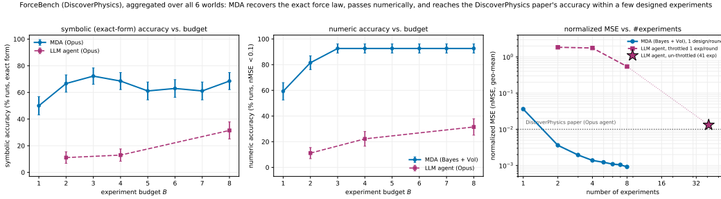
Figure 9: Numeric and symbolic data efficiency on FORCEBENCH (Opus 4.7; the numeric-only, multi-base-model version is Fig. 2). (left) Symbolic (exact-form) accuracy vs. budget: MDA (blue) vs. the pure LLM agent (purple). (middle) Numeric accuracy (nMSE < 0.1): MDA reaches \sim 93\% ; the agent \sim 31\% . (right) nMSE vs. number of experiments, with the un-throttled Opus agent (star) reproducing the DiscoverPhysics paper’s \sim 0.01 at its native \sim 41 -experiment budget. Error bars are \pm 1 SE over the 6 \times 9 runs.
