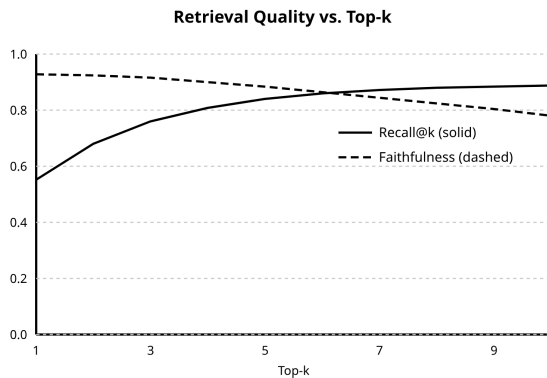
Fig. 5. Expected retrieval quality vs. top-k passages retrieved.
