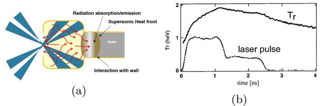
FIG. 1. (a) Experimental platform: laser beams enter the hohlraum through the LEH, generate x rays, and drive a Marshak wave in low-density foam targets of different lengths [7]. (b) Measured hohlraum drive temperature T_D(t) for the high-energy Back experiment; the dashed curve is the normalized laser pulse shape [5].
