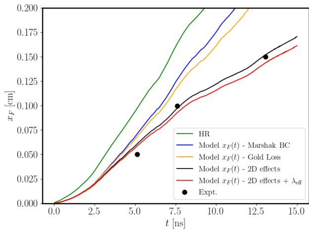
FIG. 2. Front-position comparison for the \text{SiO}_2 low-energy case, illustrating the effect of the corrected 1D and 2D terms.
