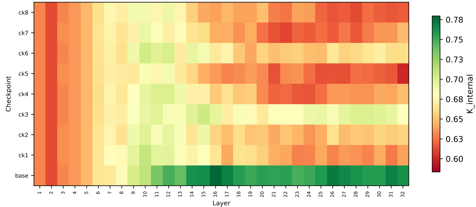
K Score (LR, own) — RMU-LAT bio
