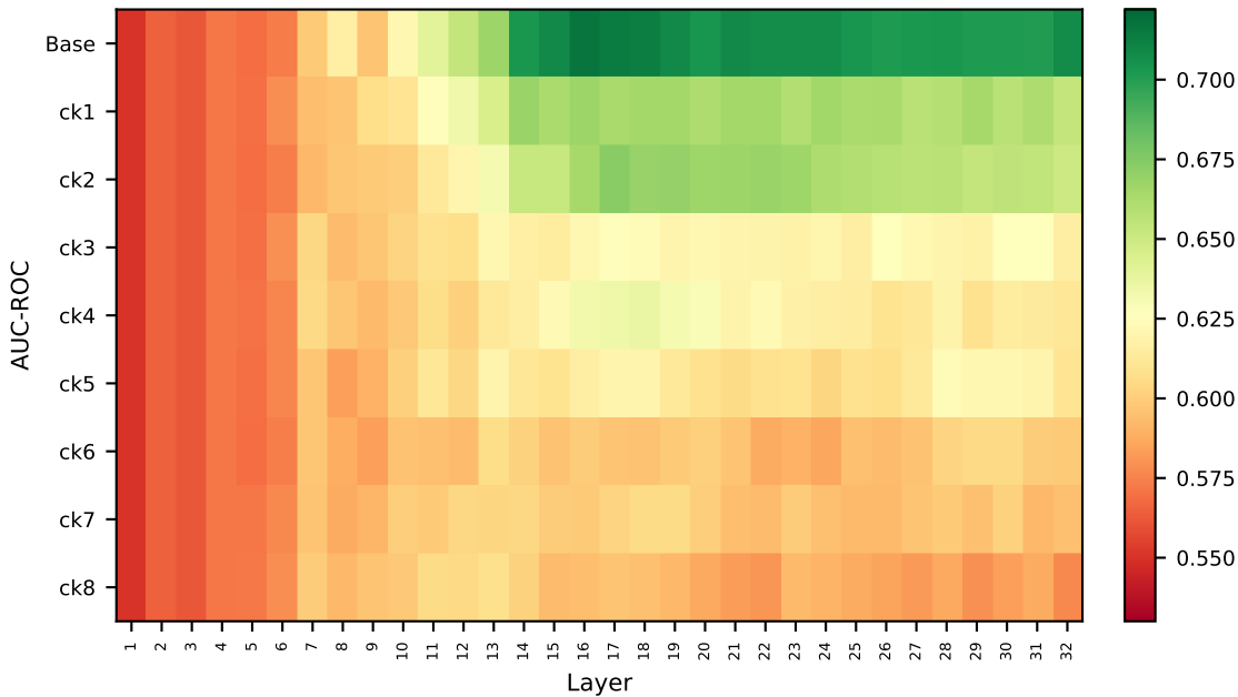
ELM — Probe Heatmap Over Training Checkpoints [Method Probes] [BIO] [LR]
