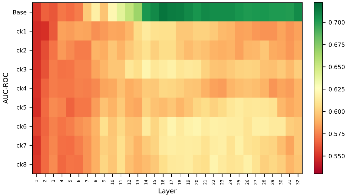
TAR — Probe Heatmap Over Training Checkpoints [Method Probes] [BIO] [LR]
