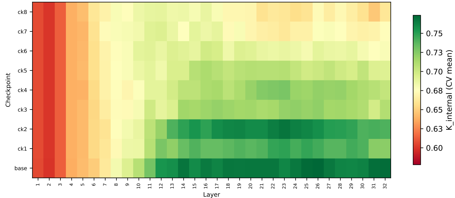
K Score CV Mean (LR) — ELM bio
