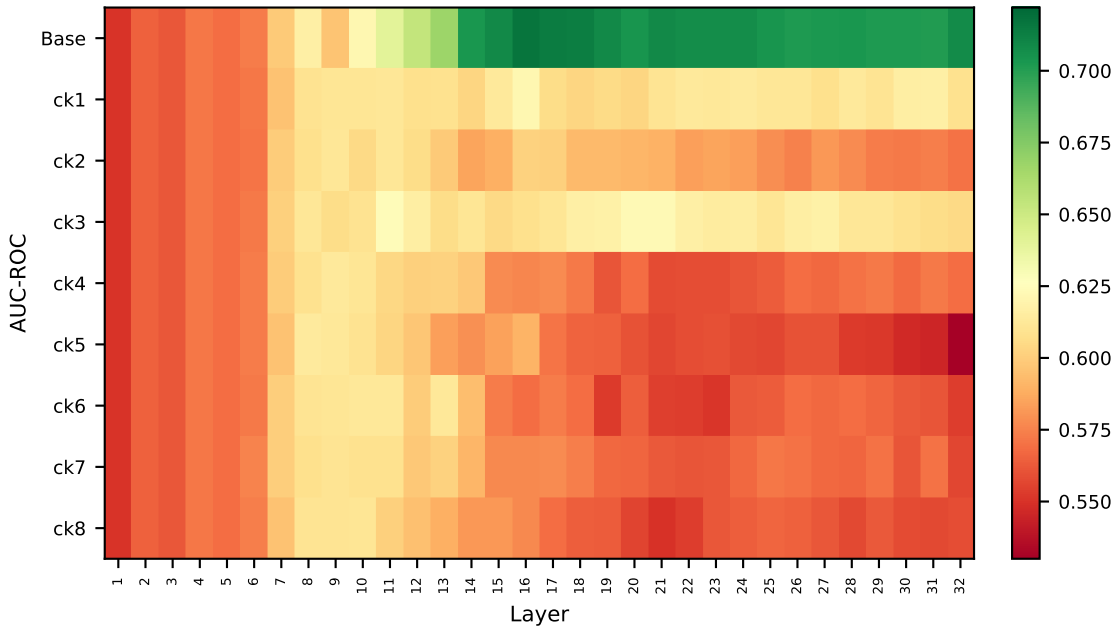
RMU — Probe Heatmap Over Training Checkpoints [Method Probes] [BIO] [LR]
