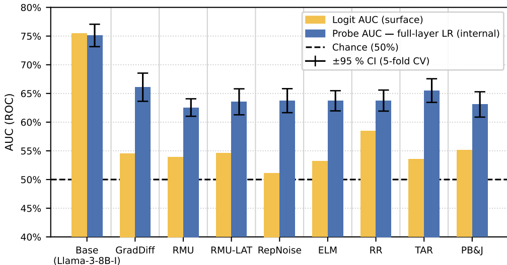
Hidden Knowledge After Unlearning — Bio (WMDP) Surface behaviour vs. internal hidden-state probe [AUC] (probe = 5-fold CV mean \pm 95 % CI)
