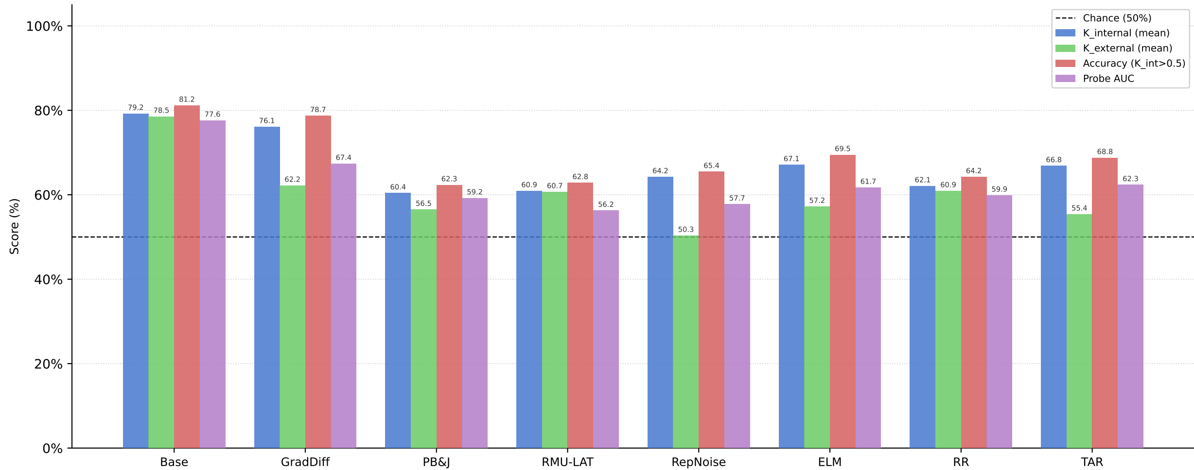
Inside-Out Probing — Base vs. ck8 Methods (bio, LR, full layer)
