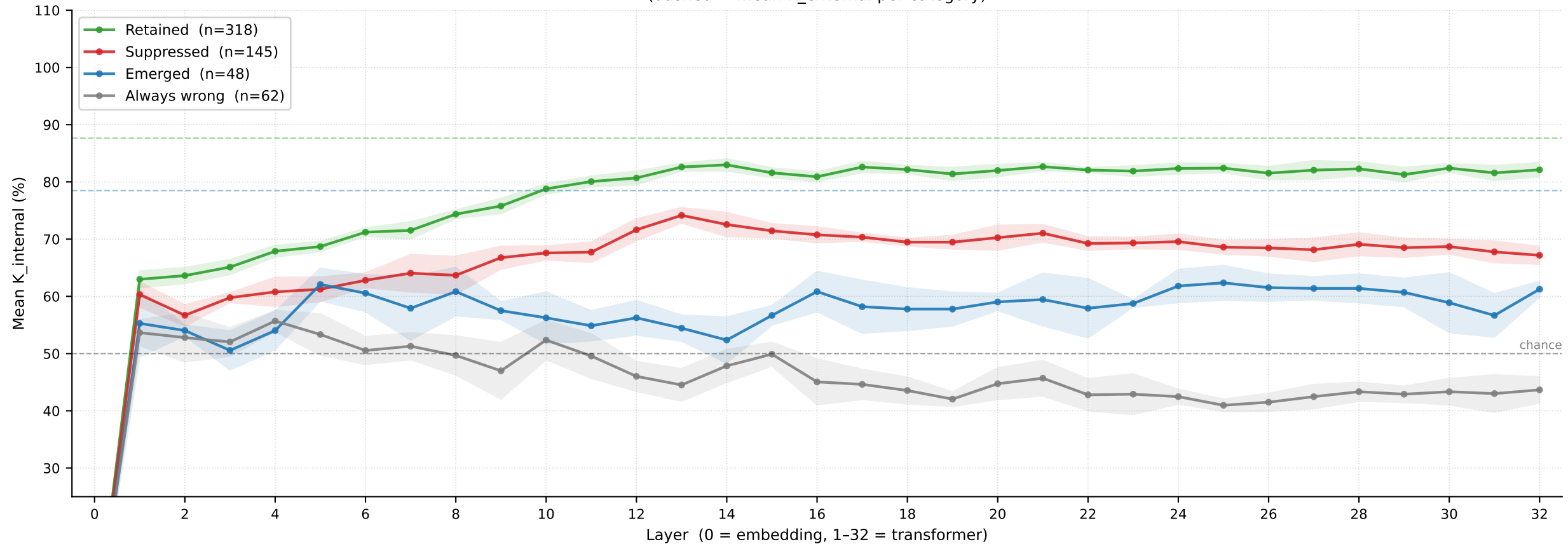
Per-layer K internal by question category — GradDiff · Bio · LR · 5-fold CV (dashed = mean K external per category)
