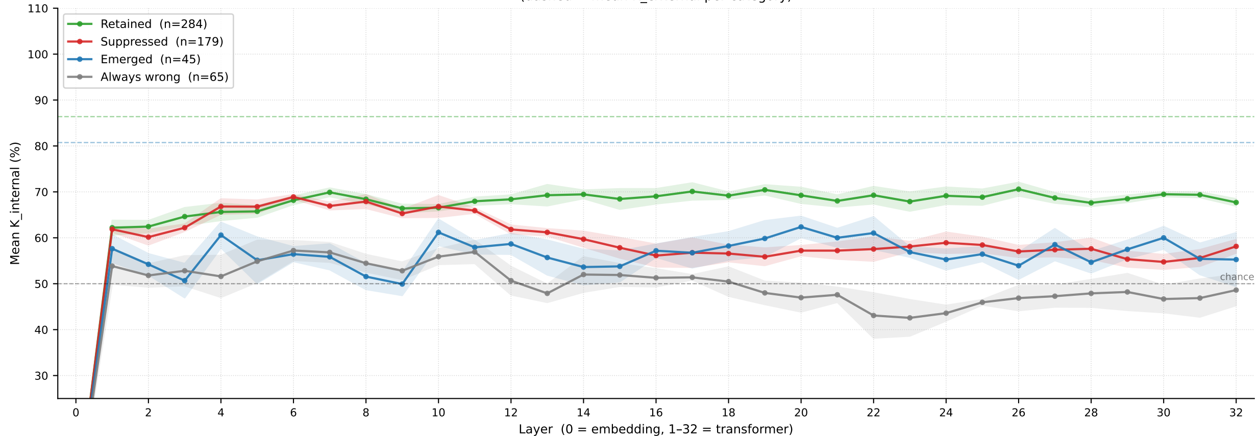
Per-layer K internal by question category — PB&J · Bio · LR · 5-fold CV (dashed = mean K external per category)
