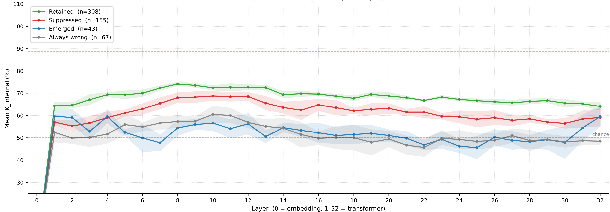
Per-layer K internal by question category — RMU-LAT · Bio · LR · 5-fold CV (dashed = mean K external per category)
