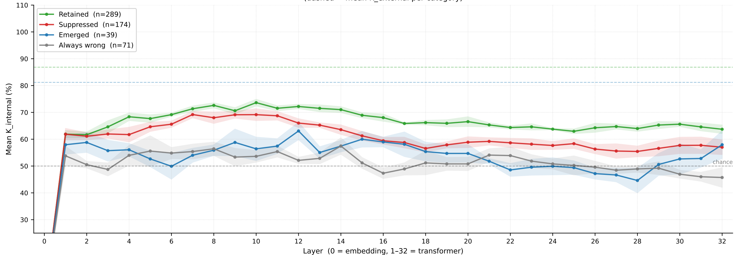
Per-layer K internal by question category — RMU · Bio · LR · 5-fold CV (dashed = mean K external per category)
