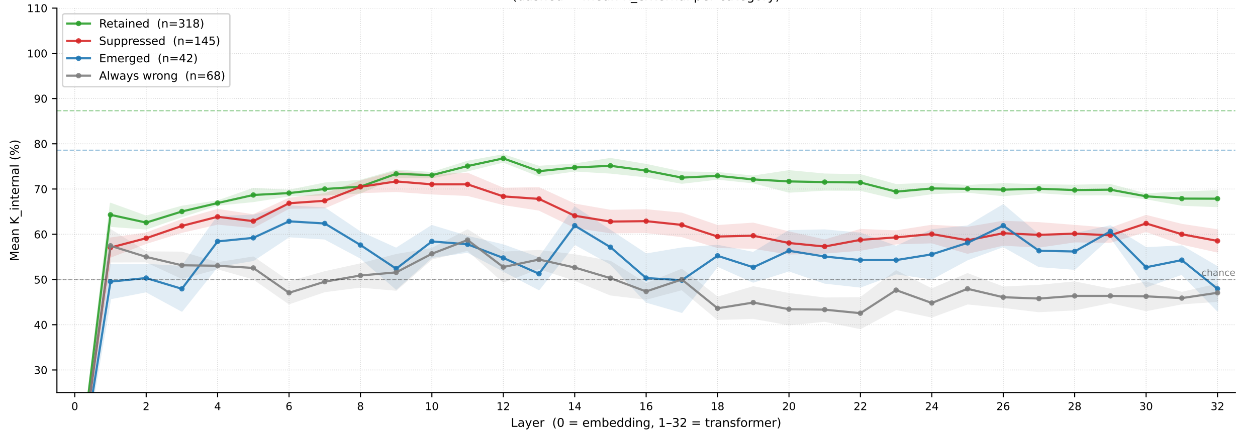
Per-layer K internal by question category — RR · Bio · LR · 5-fold CV (dashed = mean K external per category)
