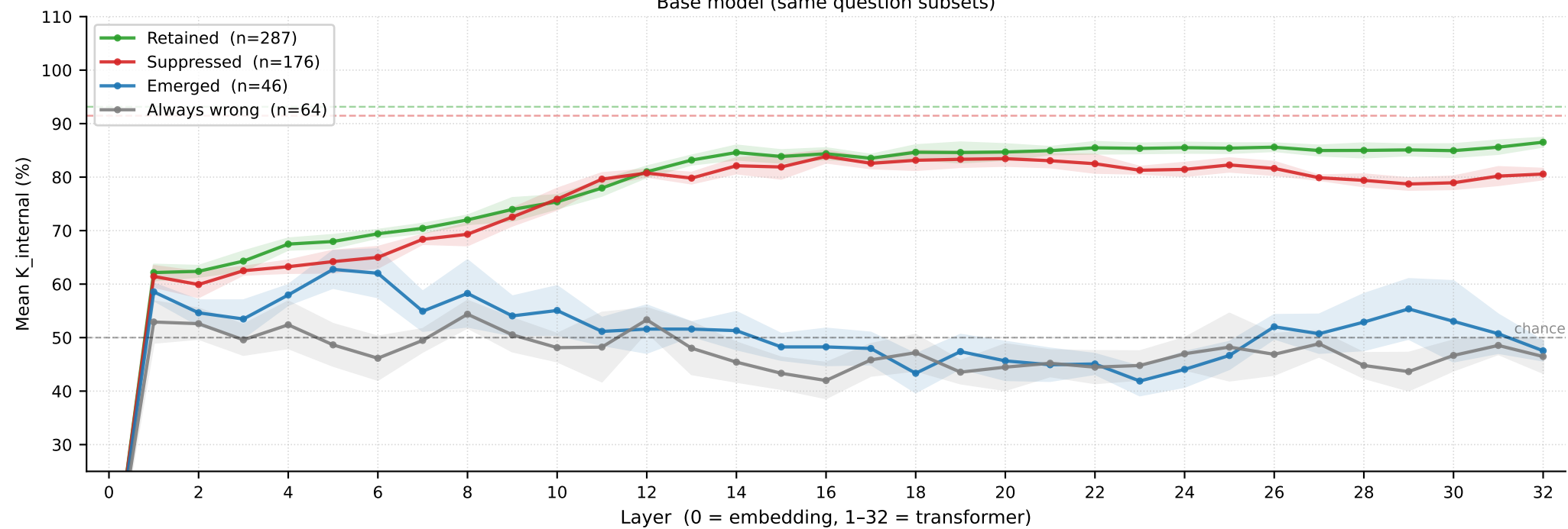
Base model (same question subsets)
