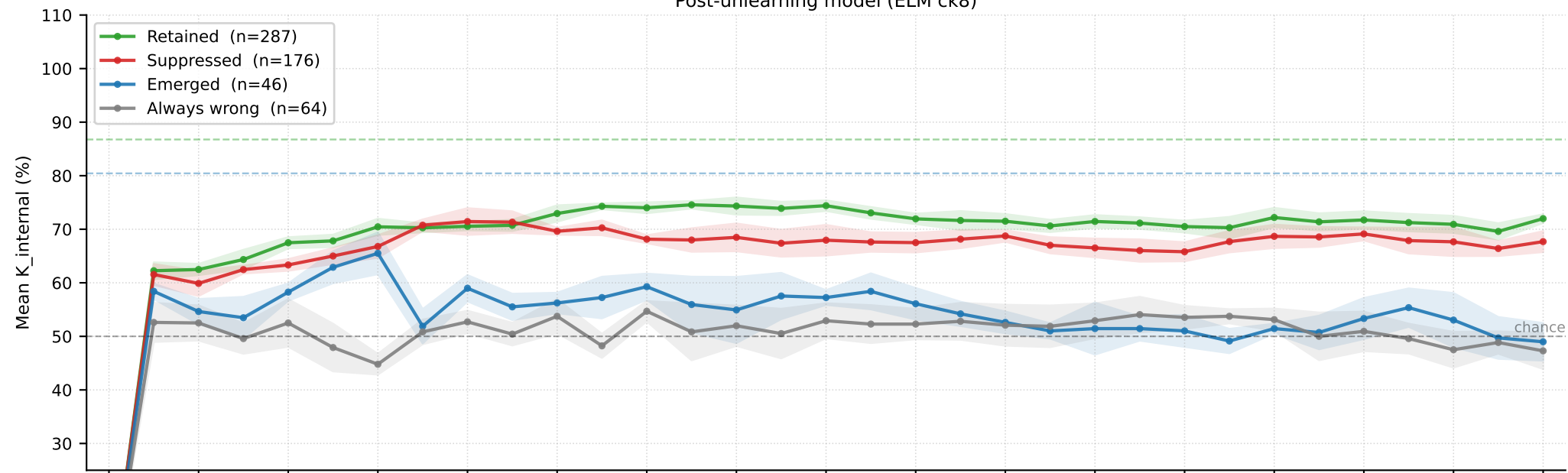
Per-layer K internal by question category — ELM · Bio · LR · 5-fold CV (dashed = mean K external per category on that model) Post-unlearning model (ELM ck8)
