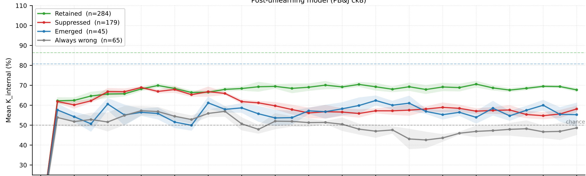
Per-layer K internal by question category — PB&J · Bio · LR · 5-fold CV (dashed = mean K external per category on that model) Post-unlearning model (PB&J ck8)
