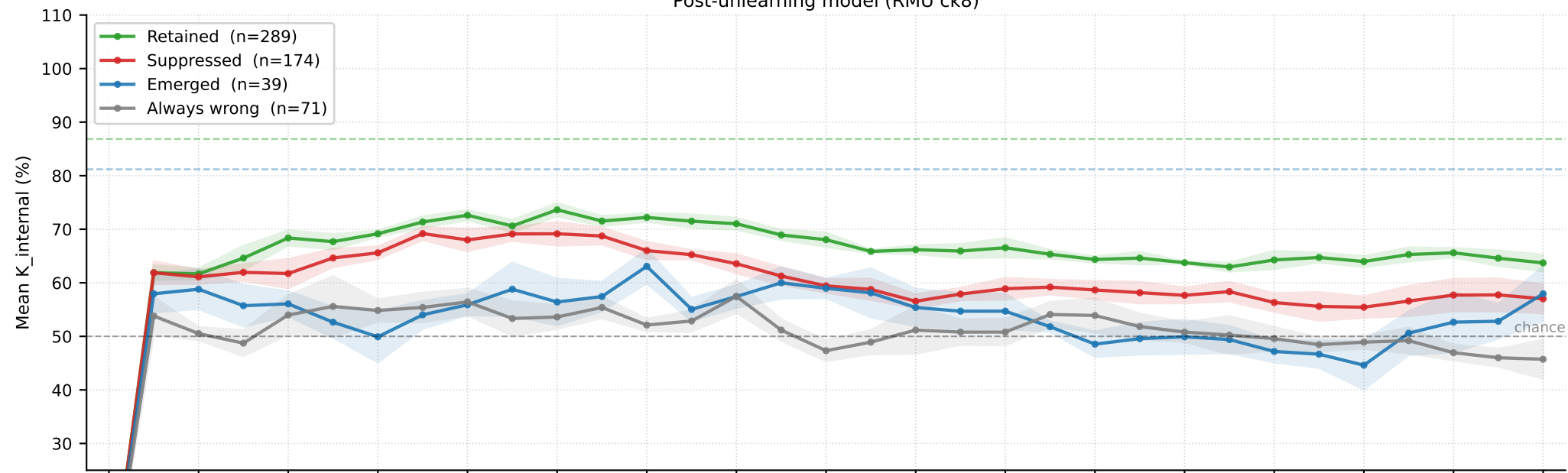
Per-layer K internal by question category — RMU · Bio · LR · 5-fold CV (dashed = mean K external per category on that model) Post-unlearning model (RMU ck8)
