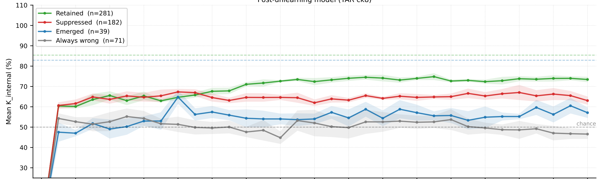
Per-layer K internal by question category — TAR · Bio · LR · 5-fold CV (dashed = mean K external per category on that model) Post-unlearning model (TAR ck8)
