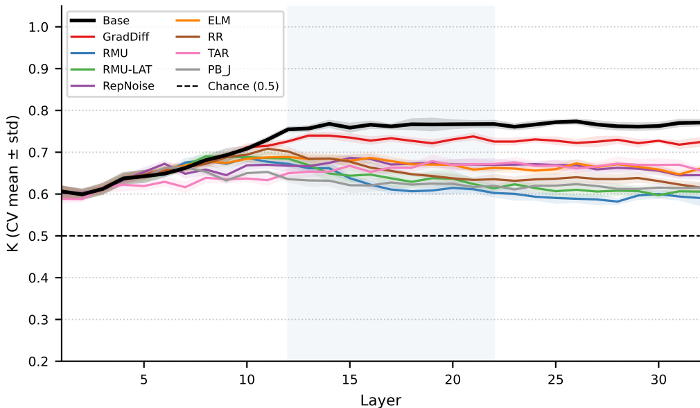
Per-Layer K Score (5-Fold CV) — bio [LR]
