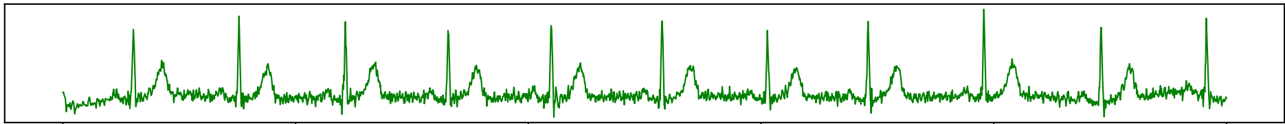
Frequency dropout
