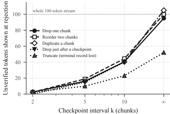
(b) Exposure when an attack is caught
