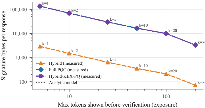
(a) Signature bytes vs. exposure
