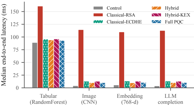
(a) End-to-end latency at 10 connections
