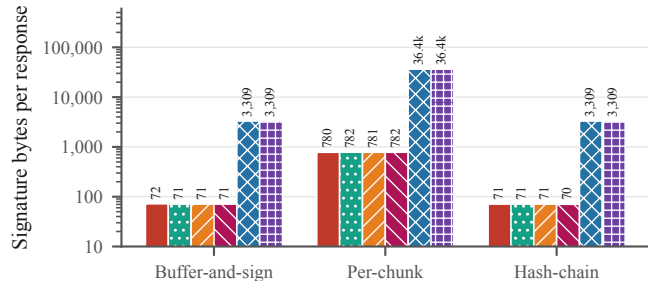
(b) Signature bytes: 50-token response
