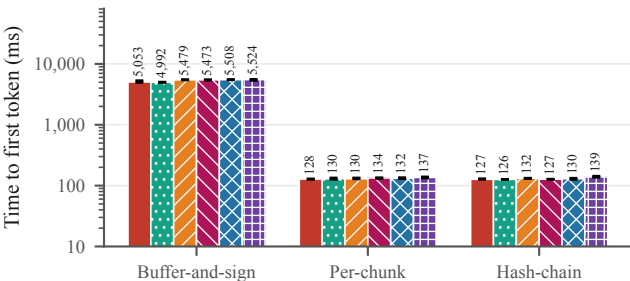
(c) Time to first token: 200-token response
