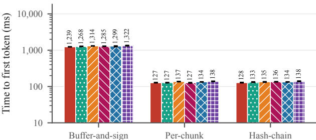
(a) Time to first token: 50-token response
