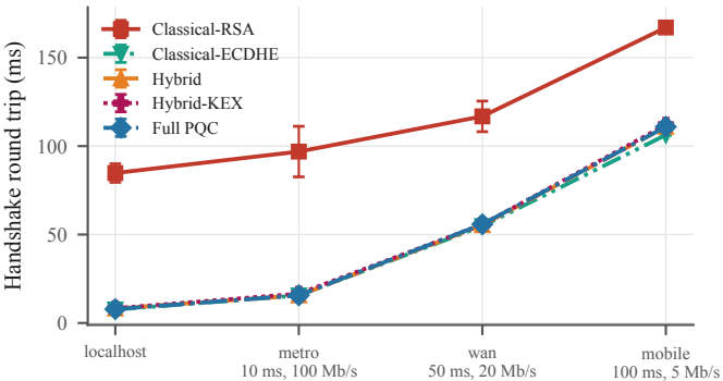
(a) Handshake leg under emulated network paths
