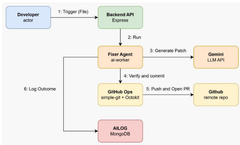
Collaboration diagram
