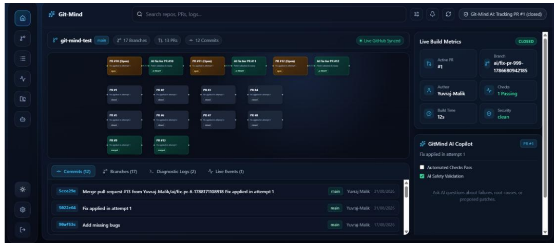
Frontend design
