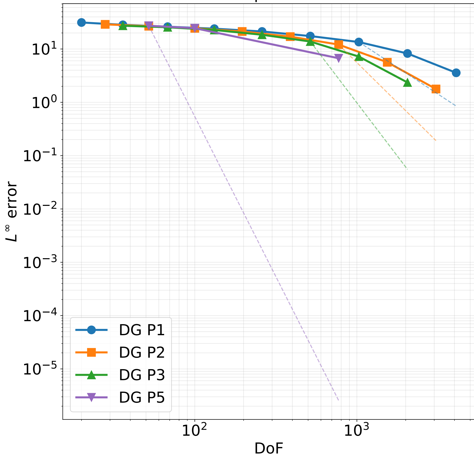
LRM SMA 4-comp — L^\infty error vs DoF
