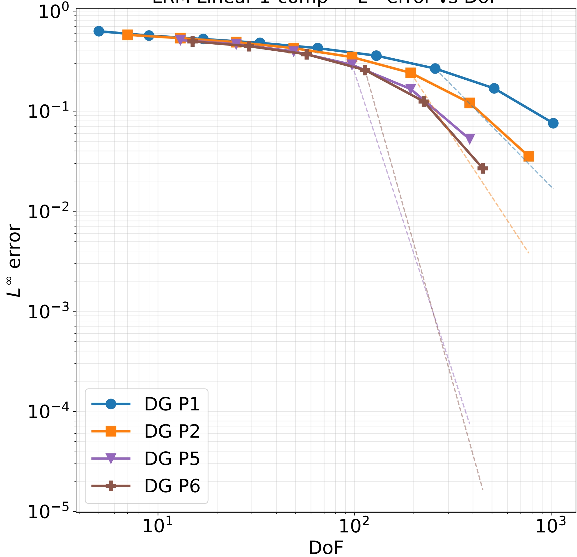
LRM Linear 1-comp — L^\infty error vs DoF
