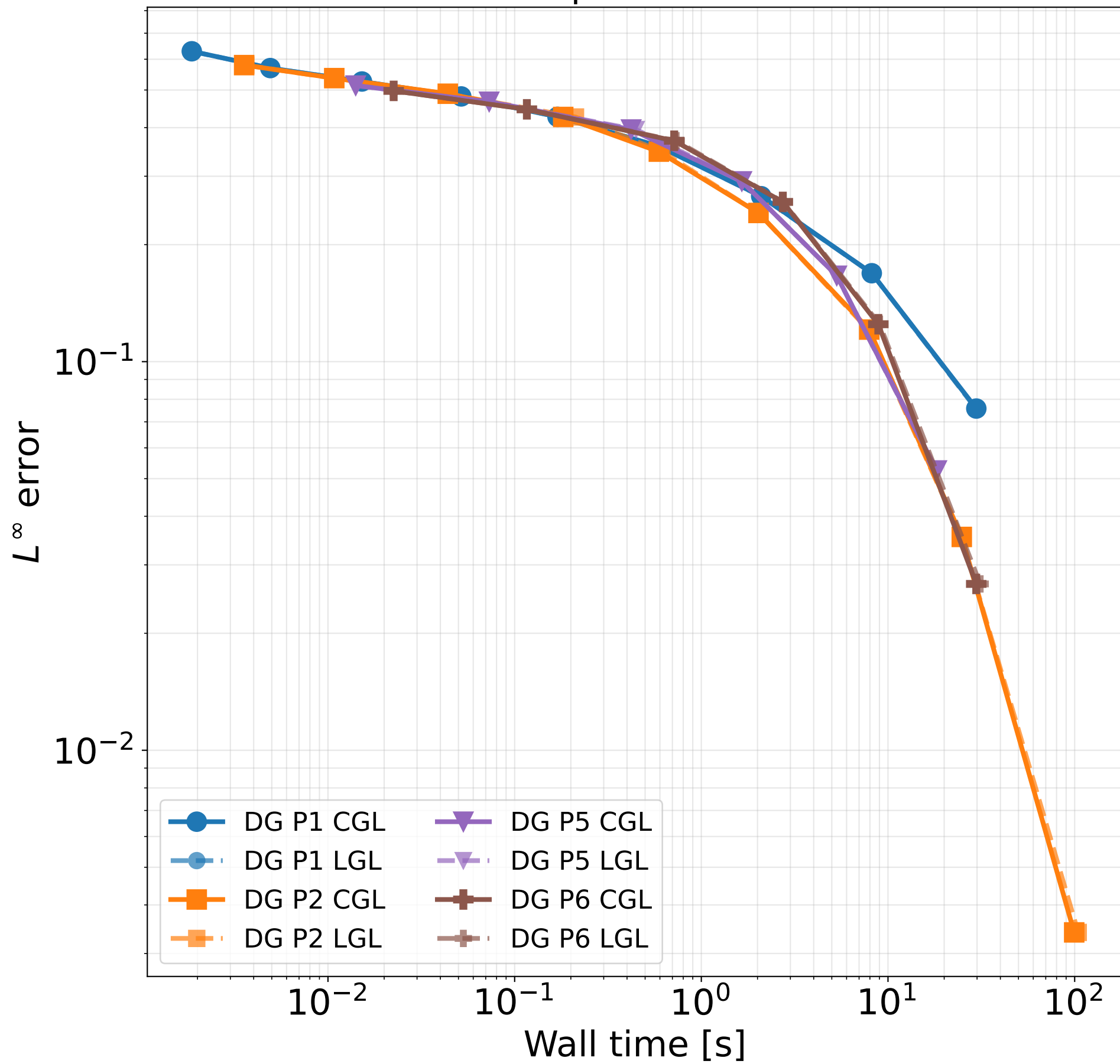
LRM Linear 1-comp — L^\infty error vs wall time
