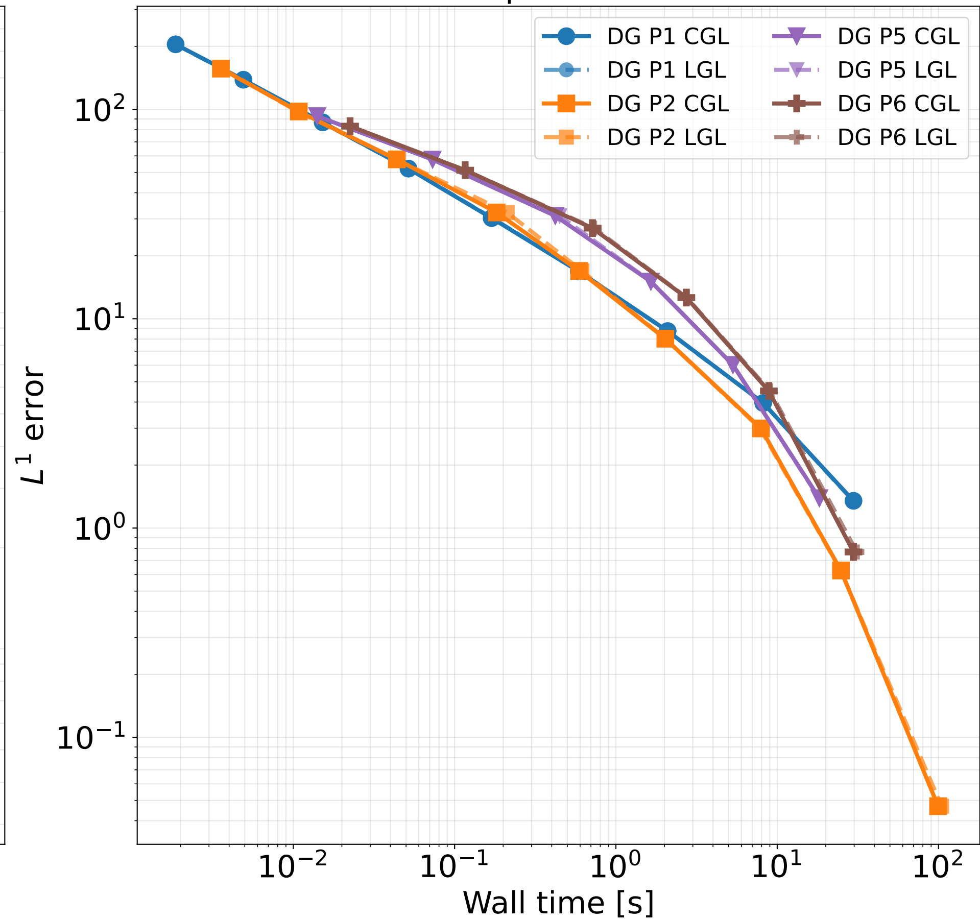
LRM Linear 1-comp — L^1 error vs wall time
