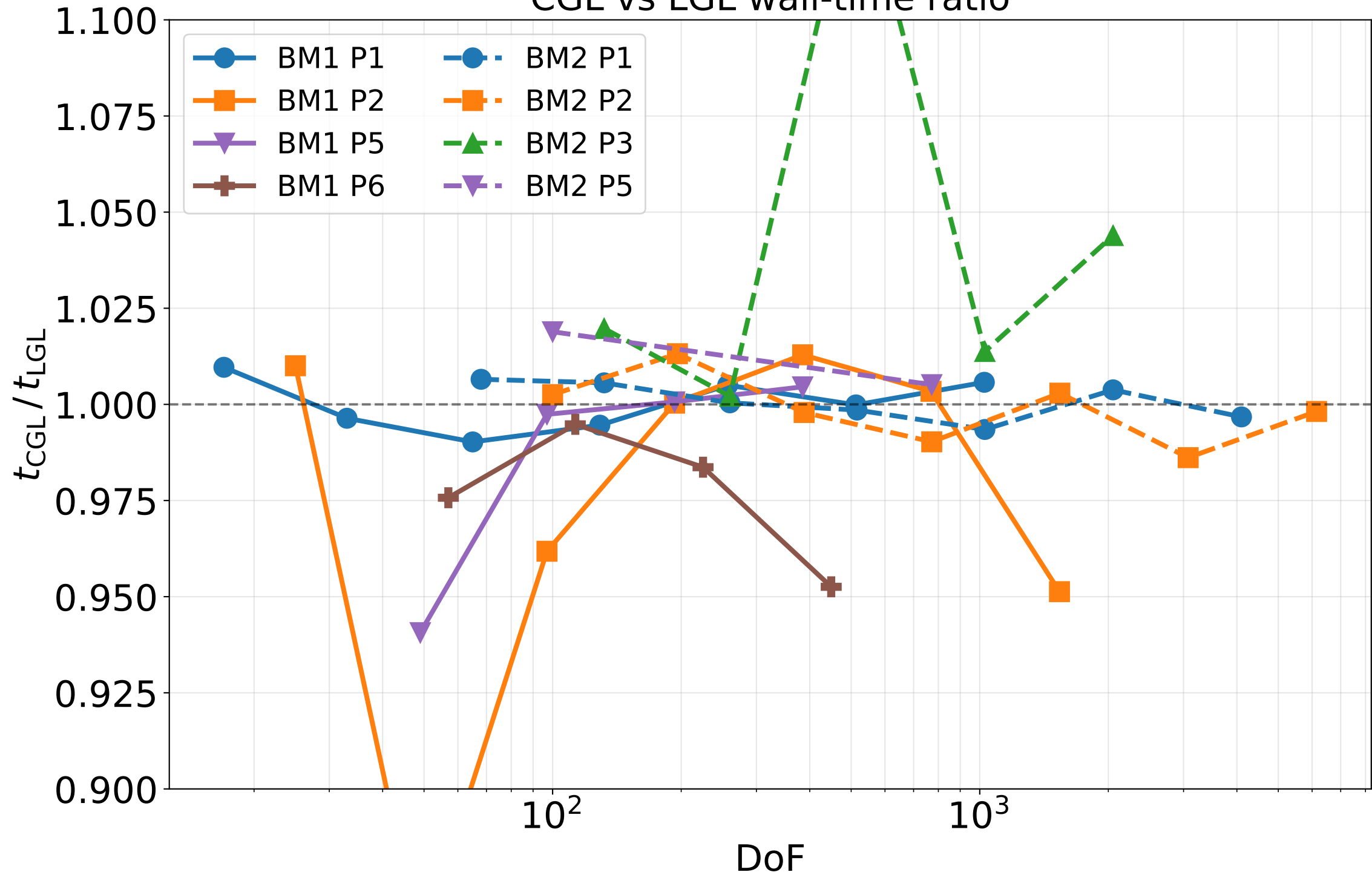
CGL vs LGL wall-time ratio
