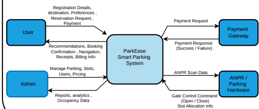
Level 0 - Context Diagram
