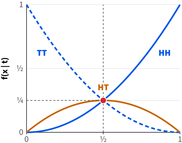
heads chance t of one coin
