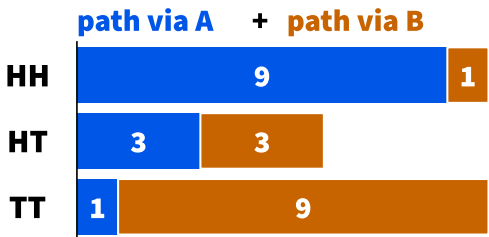
in 32nds; A's share = p(A | x) All steps: Appendix, Section 2.
