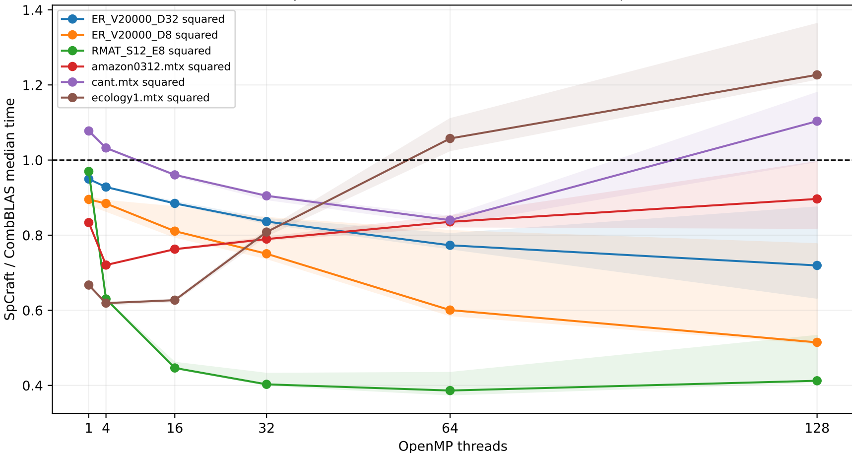
Hash SpGEMM native call time — lower favors SpCraft
