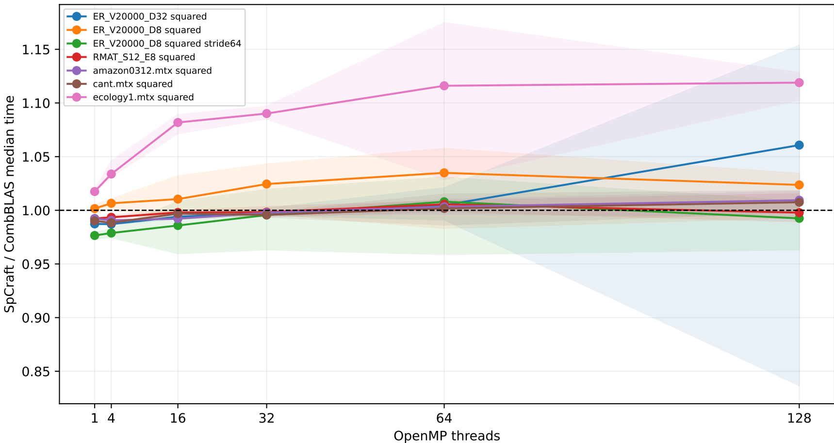
Paired DCSC-to-native-tuples hash SpGEMM
