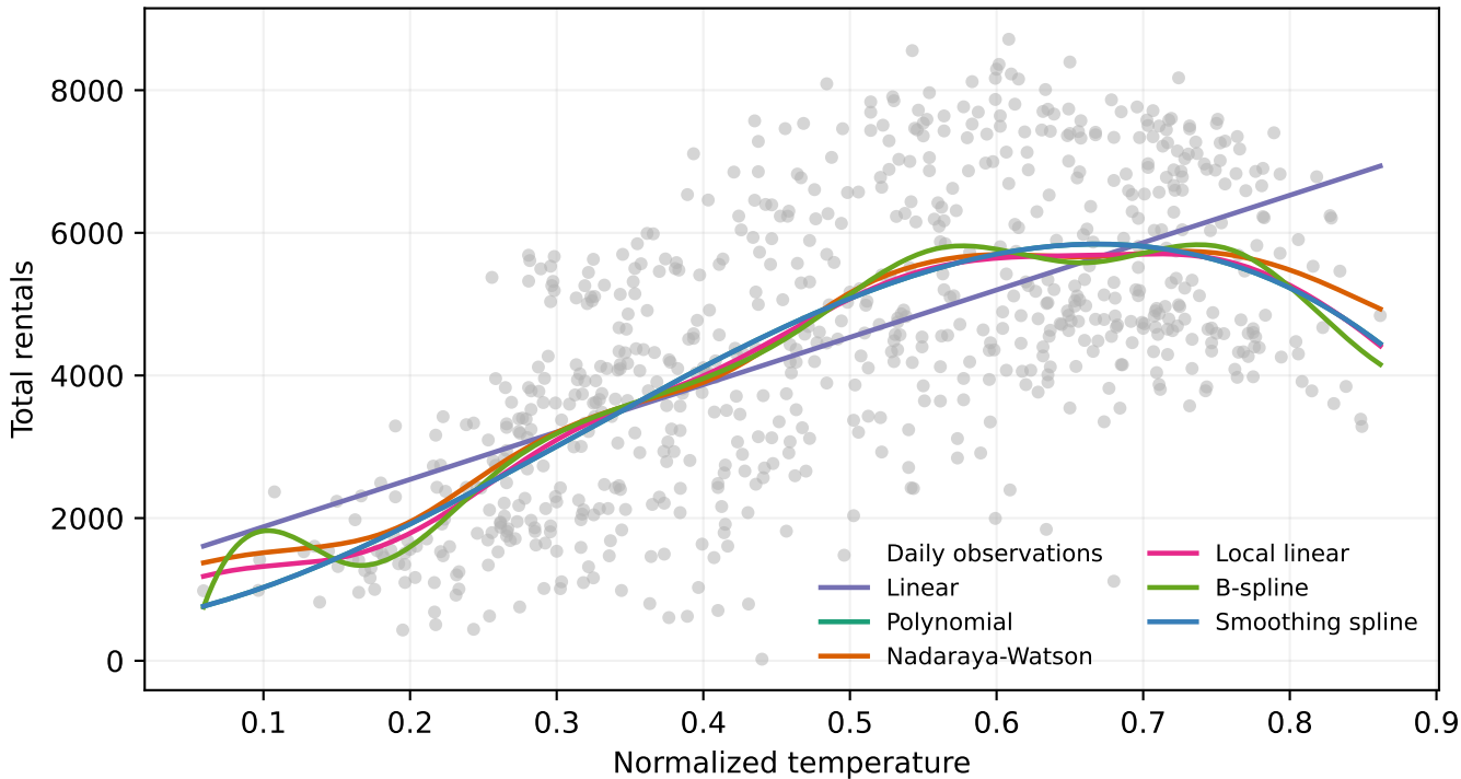
Nonparametric smoothing of total rentals by temperature
