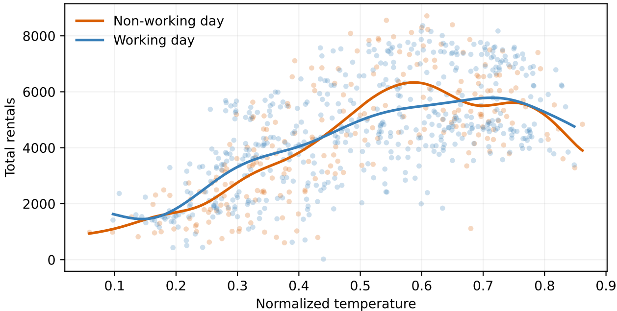
Local linear fits by working-day status
