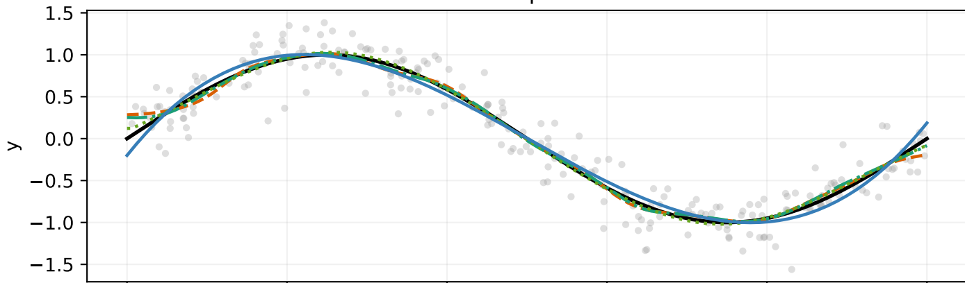
Local spike
