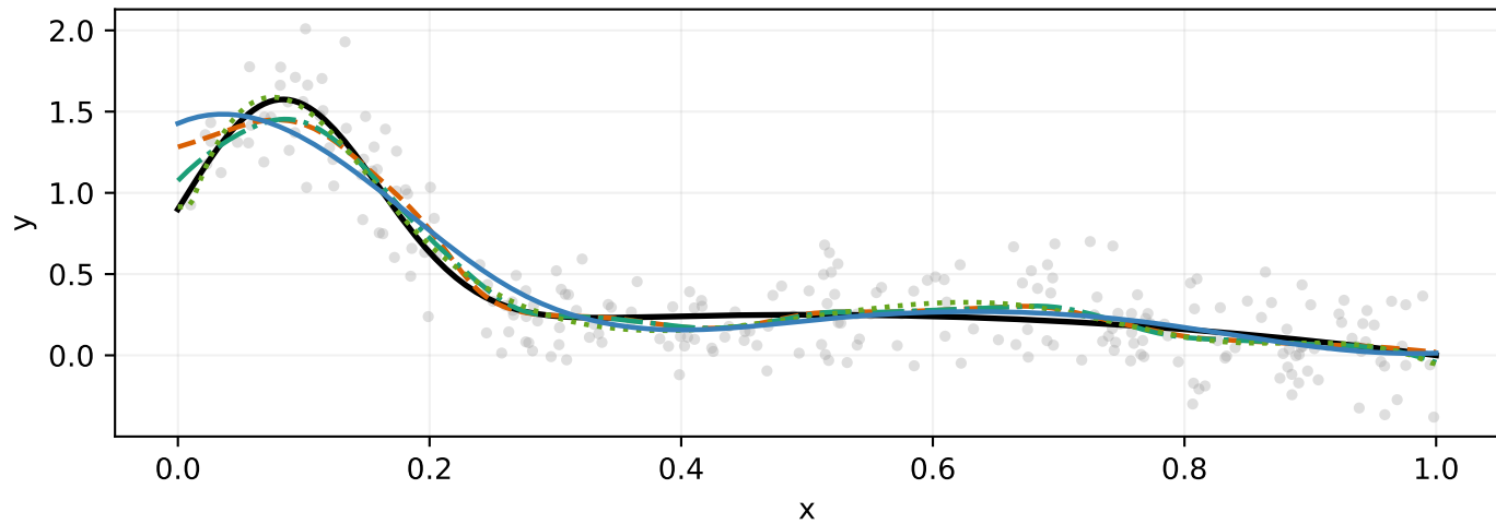
Boundary change
