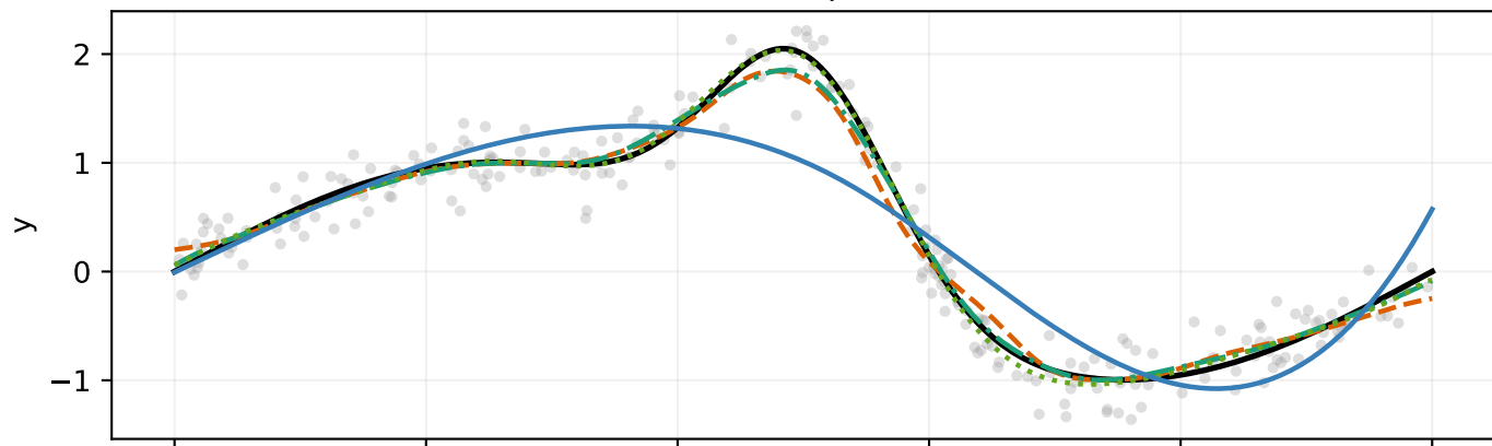
Boundary change
