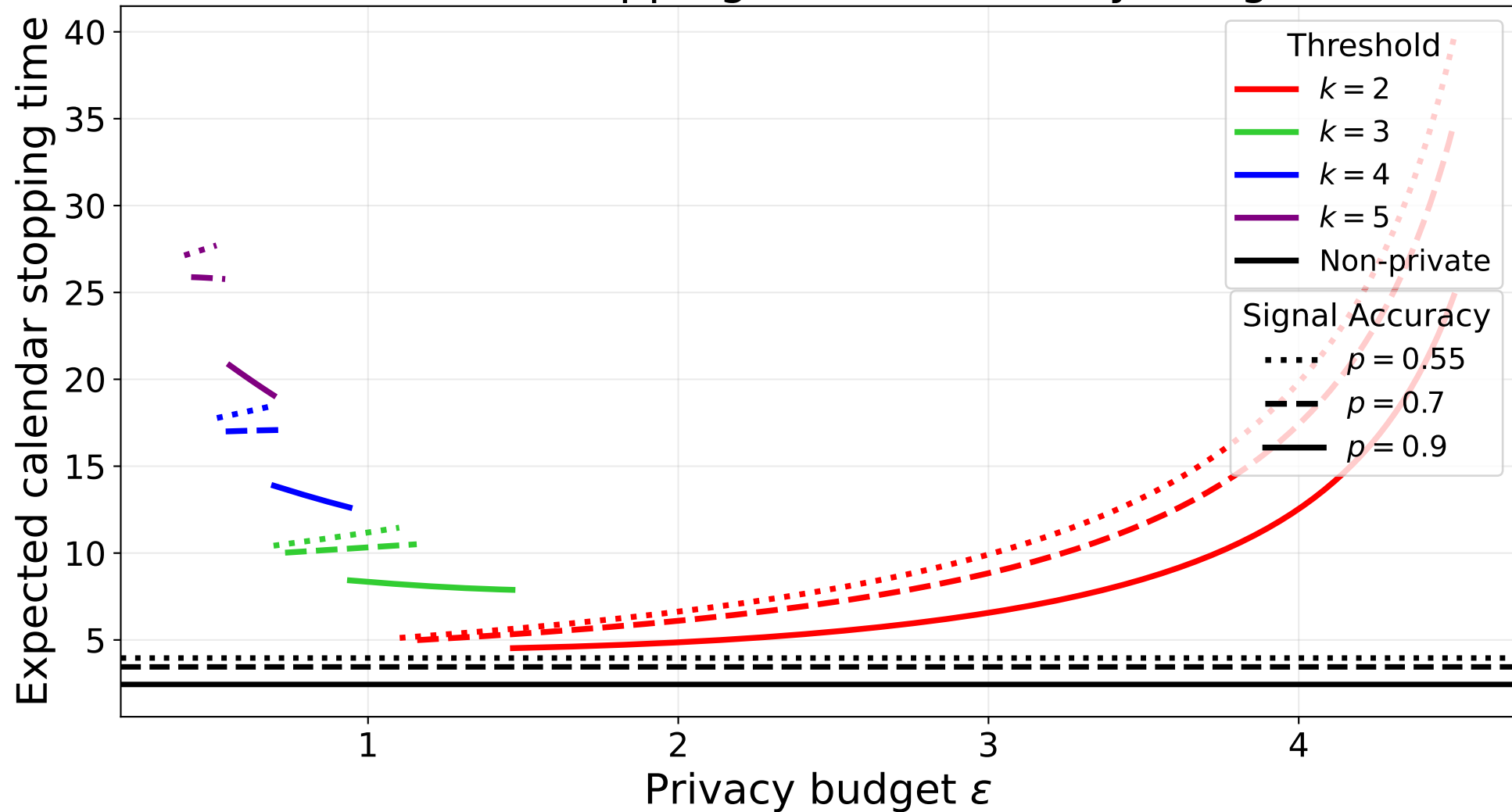
Calendar Stopping Time vs. Privacy Budget
